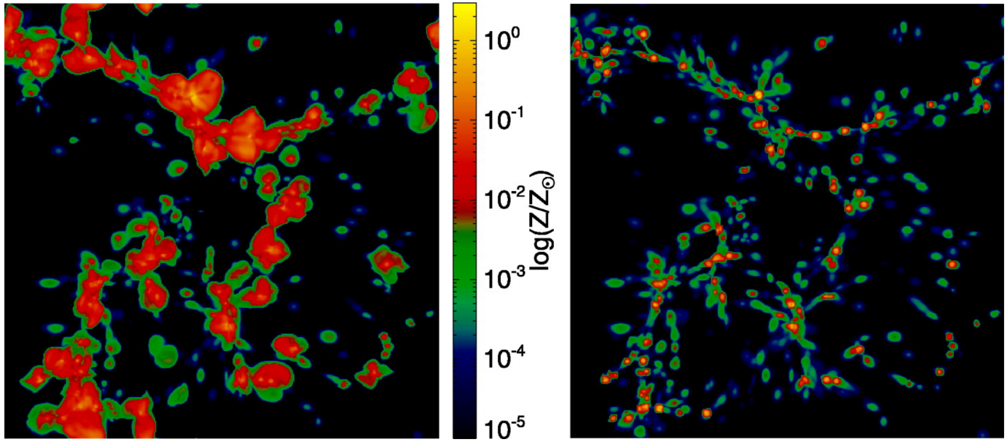
Fig. 5. from Quantitative Signatures of Galactic Superwinds on Ly Clouds and MetalLine Systems Cen, Nagamine, & Ostriker 2005 ApJ 635 86 doi:10.1086/497353 https://dx.doi.org/10.1086/497353
