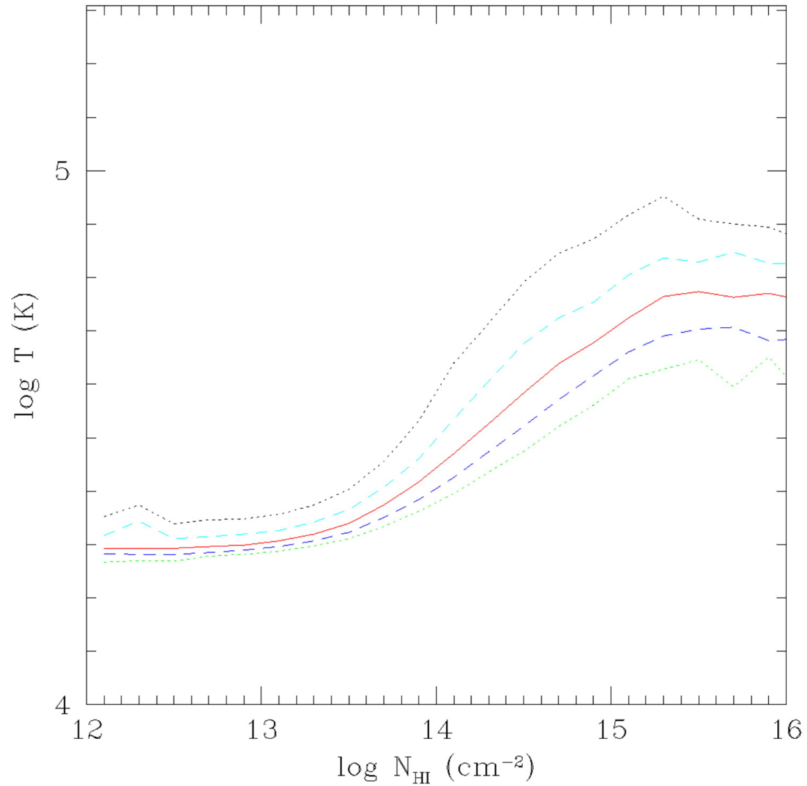
Fig. 4. from Quantitative Signatures of Galactic Superwinds on Ly Clouds and MetalLine Systems Cen, Nagamine, & Ostriker 2005 ApJ 635 86 doi:10.1086/497353 https://dx.doi.org/10.1086/497353 © 2005. The American Astronomical Society. All rights reserved. Printed in U.S.A.
