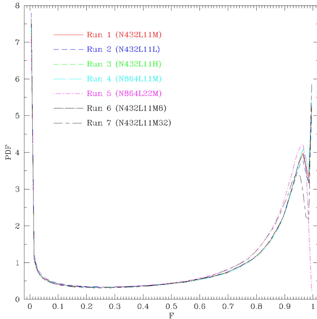
Fig. 3. from Quantitative Signatures of Galactic Superwinds on Ly Clouds and MetalLine Systems Cen, Nagamine, & Ostriker 2005 ApJ 635 86 doi:10.1086/497353 https://dx.doi.org/10.1086/497353 © 2005. The American Astronomical Society. All rights reserved. Printed in U.S.A.
