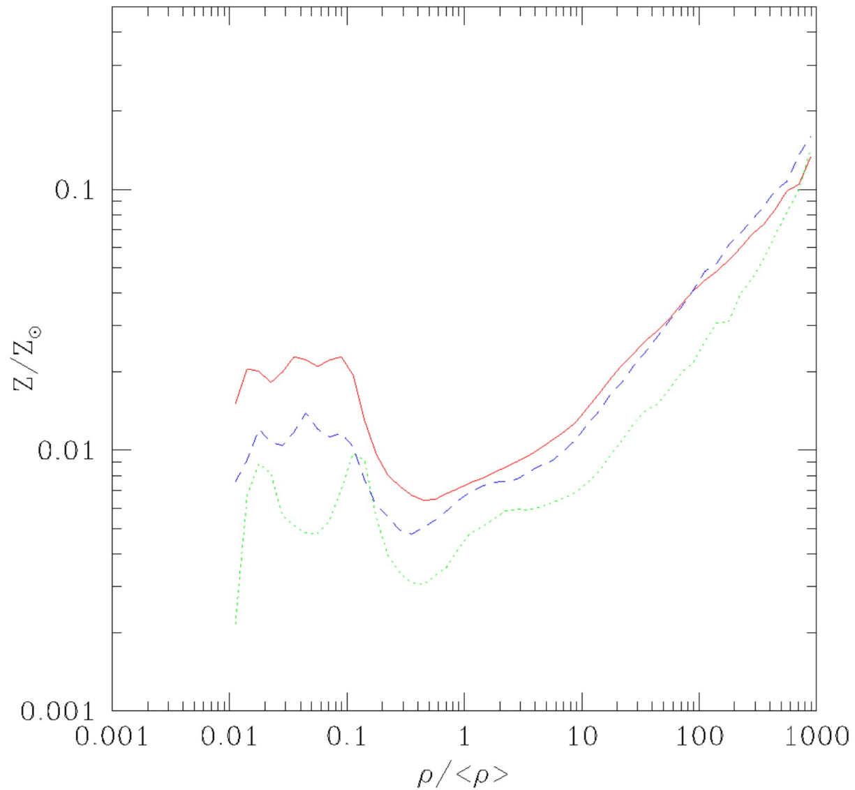
Fig. 14. from Quantitative Signatures of Galactic Superwinds on Ly Clouds and MetalLine Systems Cen, Nagamine, & Ostriker 2005 ApJ 635 86 doi:10.1086/497353 https://dx.doi.org/10.1086/497353 © 2005. The American Astronomical Society. All rights reserved. Printed in U.S.A.
