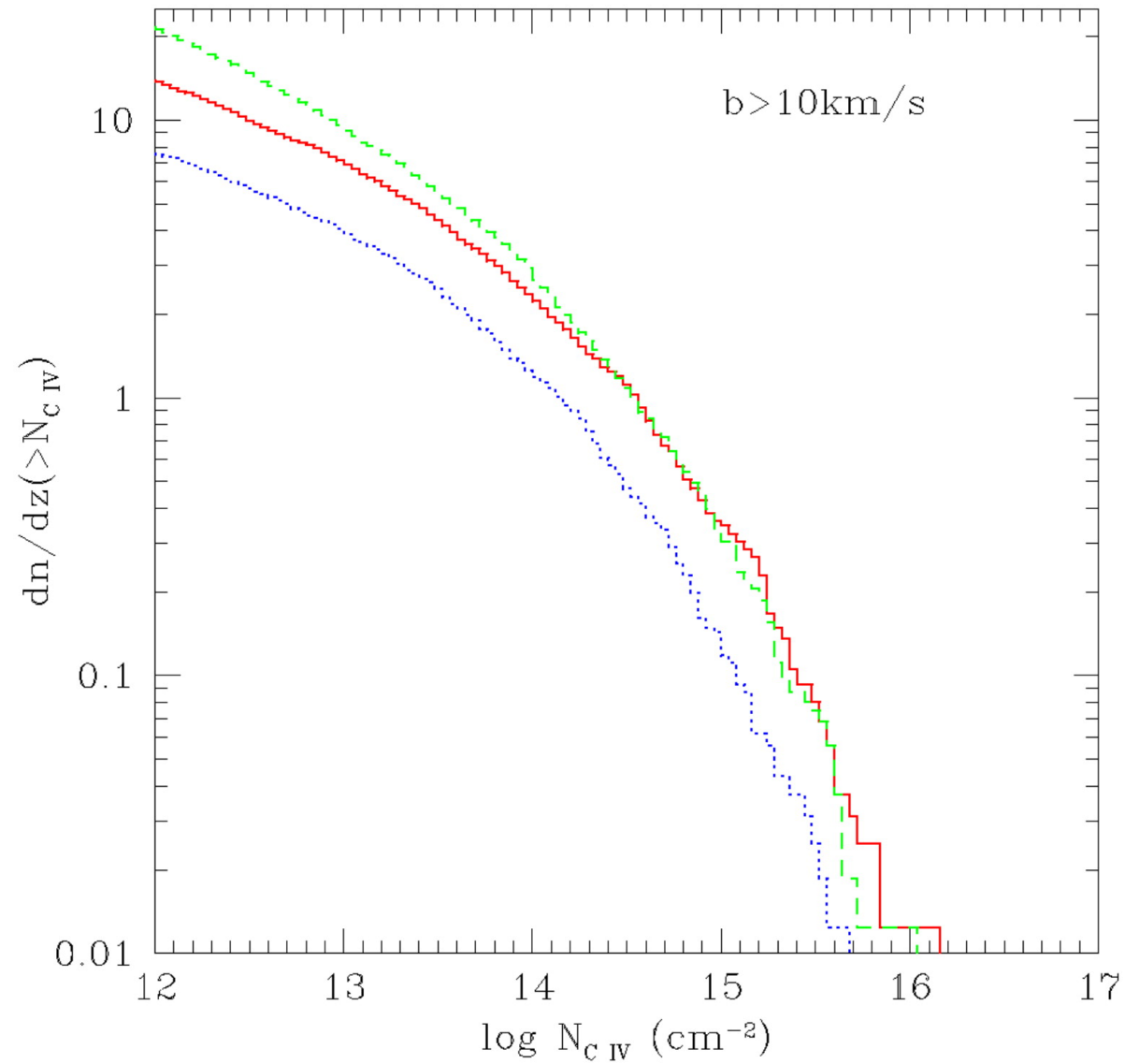
Fig. 12. from Quantitative Signatures of Galactic Superwinds on Ly Clouds and MetalLine Systems Cen, Nagamine, & Ostriker 2005 ApJ 635 86 doi:10.1086/497353 https://dx.doi.org/10.1086/497353 © 2005. The American Astronomical Society. All rights reserved. Printed in U.S.A.
