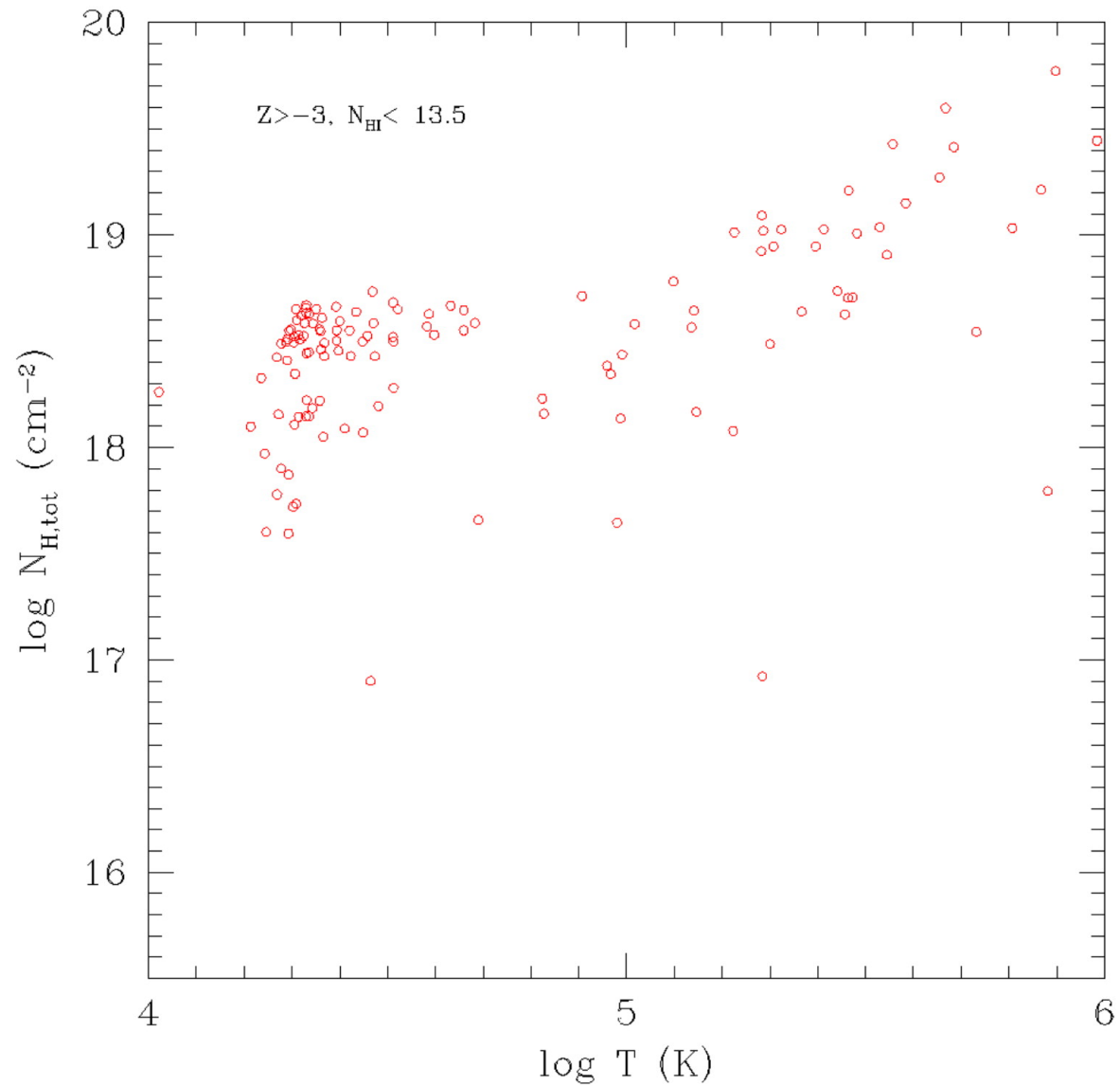
Fig. 11. from Quantitative Signatures of Galactic Superwinds on Ly Clouds and MetalLine Systems Cen, Nagamine, & Ostriker 2005 ApJ 635 86 doi:10.1086/497353 https://dx.doi.org/10.1086/497353 © 2005. The American Astronomical Society. All rights reserved. Printed in U.S.A.
