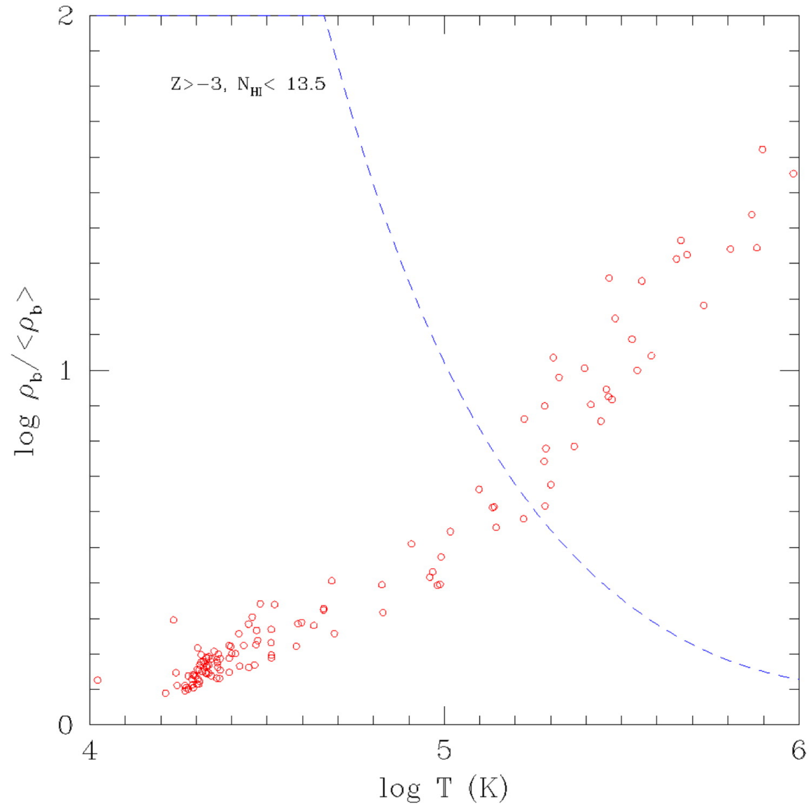
Fig. 10. from Quantitative Signatures of Galactic Superwinds on Ly Clouds and MetalLine Systems Cen, Nagamine, & Ostriker 2005 ApJ 635 86 doi:10.1086/497353 https://dx.doi.org/10.1086/497353 © 2005. The American Astronomical Society. All rights reserved. Printed in U.S.A.
