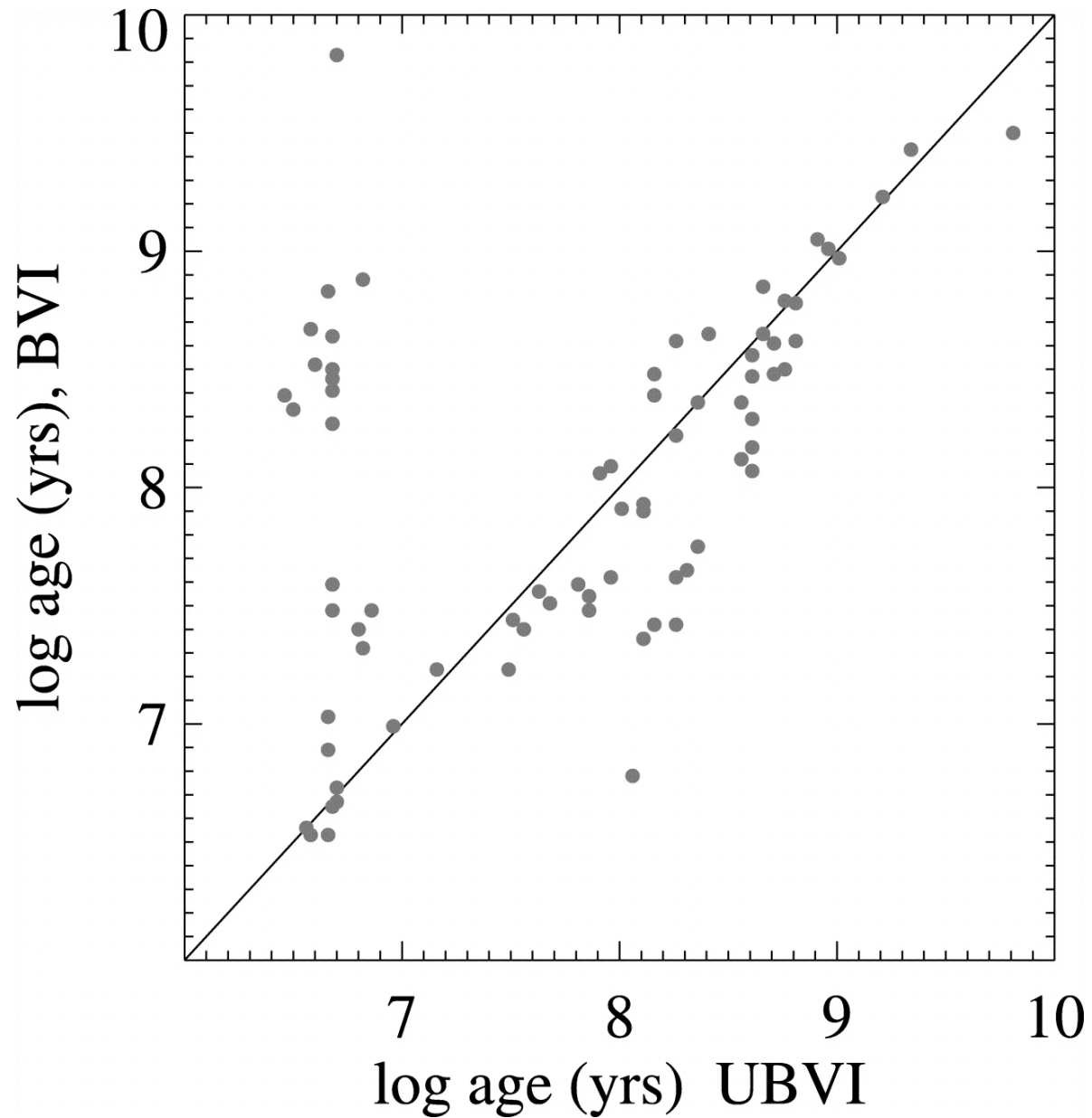
Fig. 6. from Properties of Resolved Star Clusters in M51 Lee, Chandar, & Whitmore 2005 AJ 130 2128 doi:10.1086/491786 https://dx.doi.org/10.1086/491786
