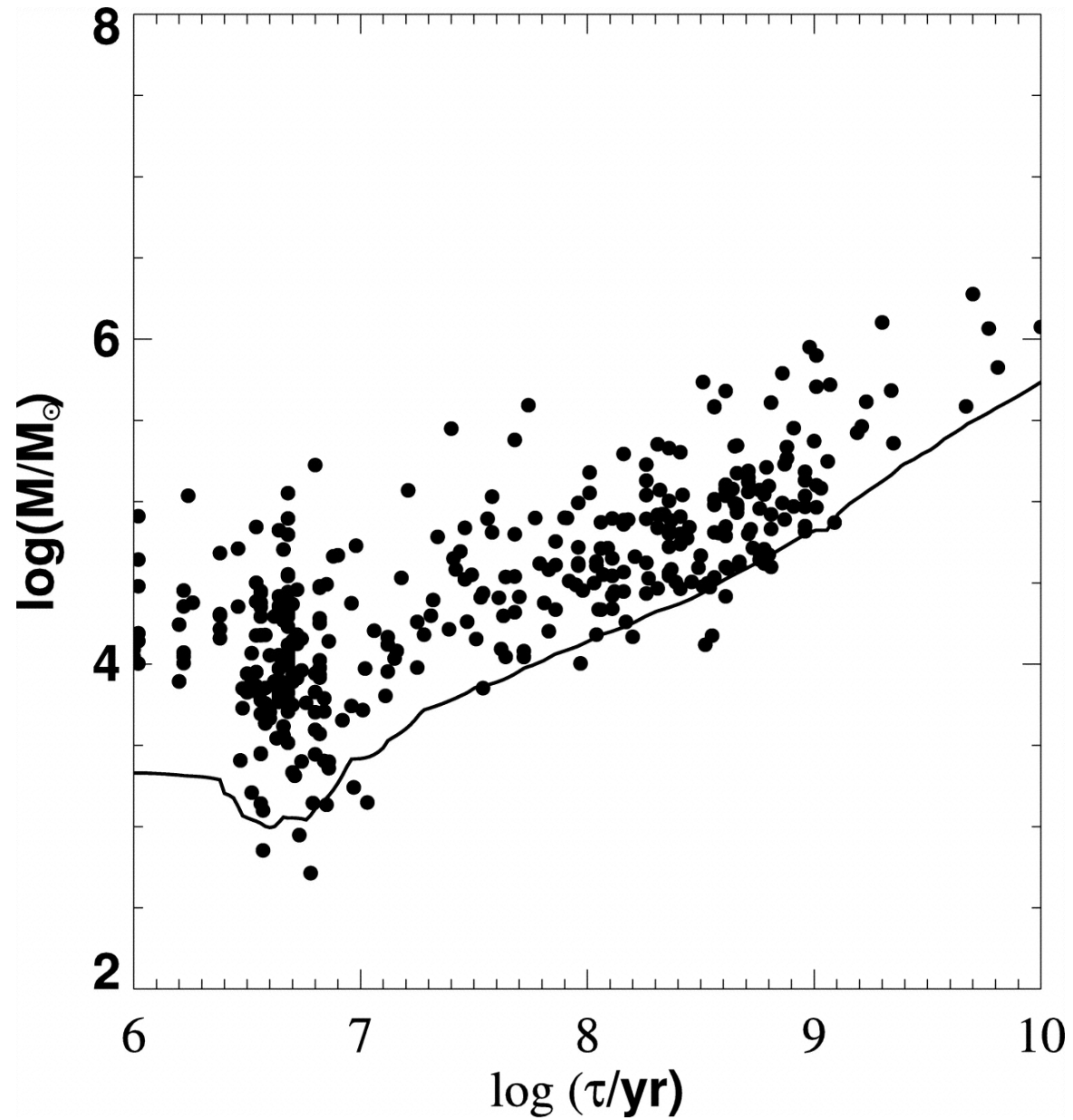
Fig. 5. from Properties of Resolved Star Clusters in M51 Lee, Chandar, & Whitmore 2005 AJ 130 2128 doi:10.1086/491786 https://dx.doi.org/10.1086/491786
