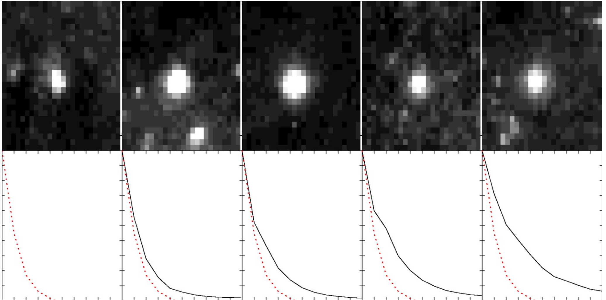
Fig. 2. from Properties of Resolved Star Clusters in M51 Lee, Chandar, & Whitmore 2005 AJ 130 2128 doi:10.1086/491786 https://dx.doi.org/10.1086/491786
