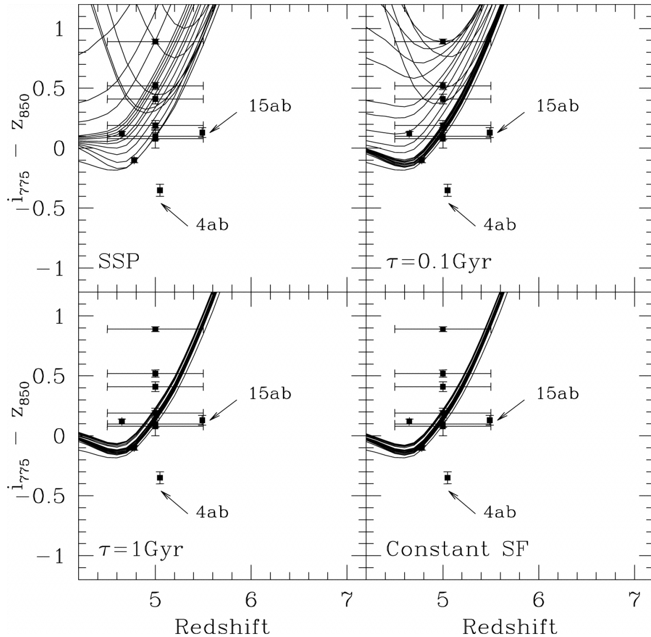
Fig. 8. from RestFrame UltraviolettoOptical Properties of Galaxies at z \sim 6 and z \sim 5 in the Hubble Ultra Deep Field: From Hubble to Spitzer Yan et al. 2005 ApJ 634 109 doi:10.1086/491695 https://dx.doi.org/10.1086/491695 © 2005. The American Astronomical Society. All rights reserved. Printed in U.S.A.
