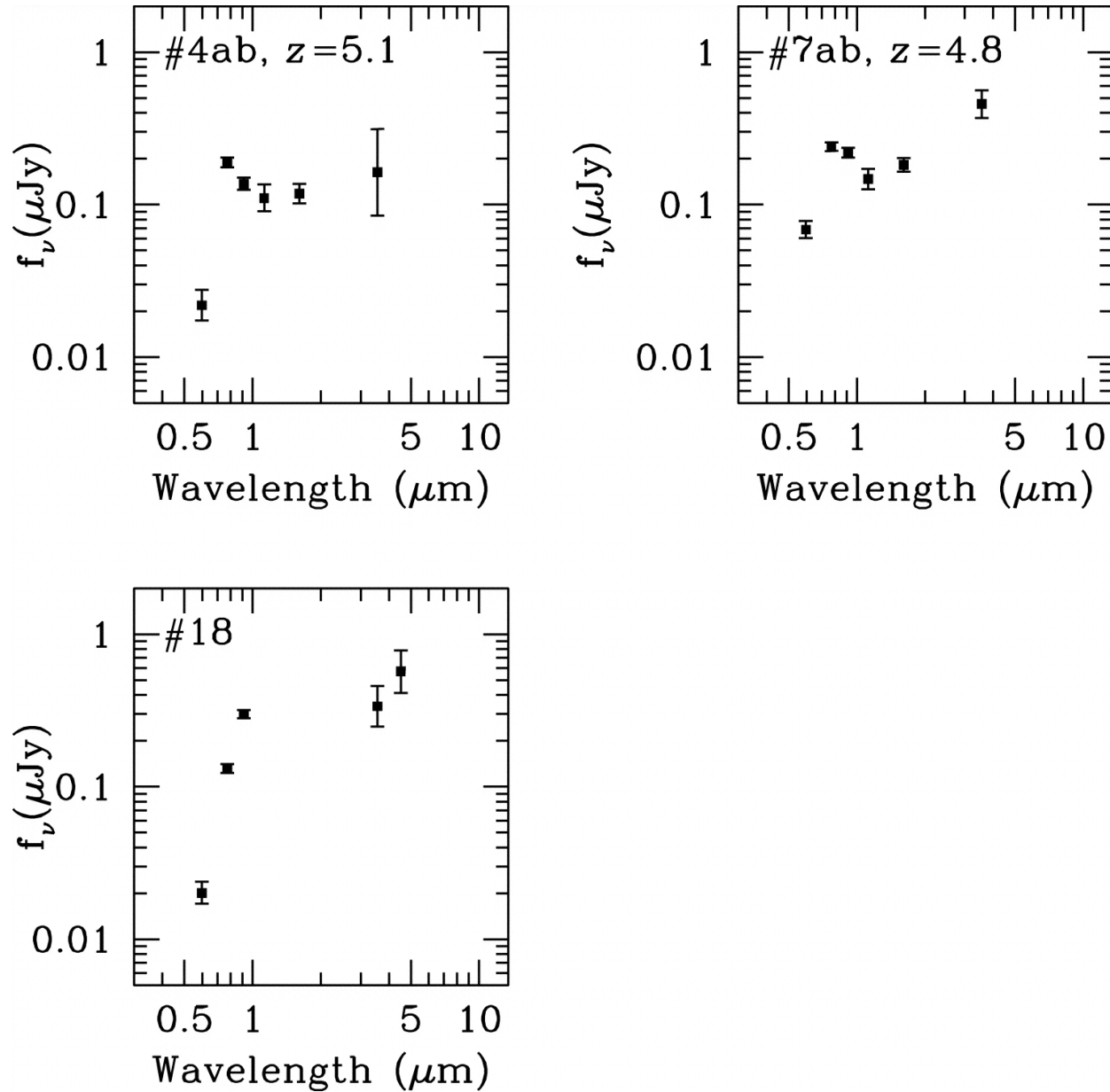
Fig. 7. from RestFrame UltraviolettoOptical Properties of Galaxies at z \sim 6 and z \sim 5 in the Hubble Ultra Deep Field: From Hubble to Spitzer Yan et al. 2005 ApJ 634 109 doi:10.1086/491695 https://dx.doi.org/10.1086/491695
