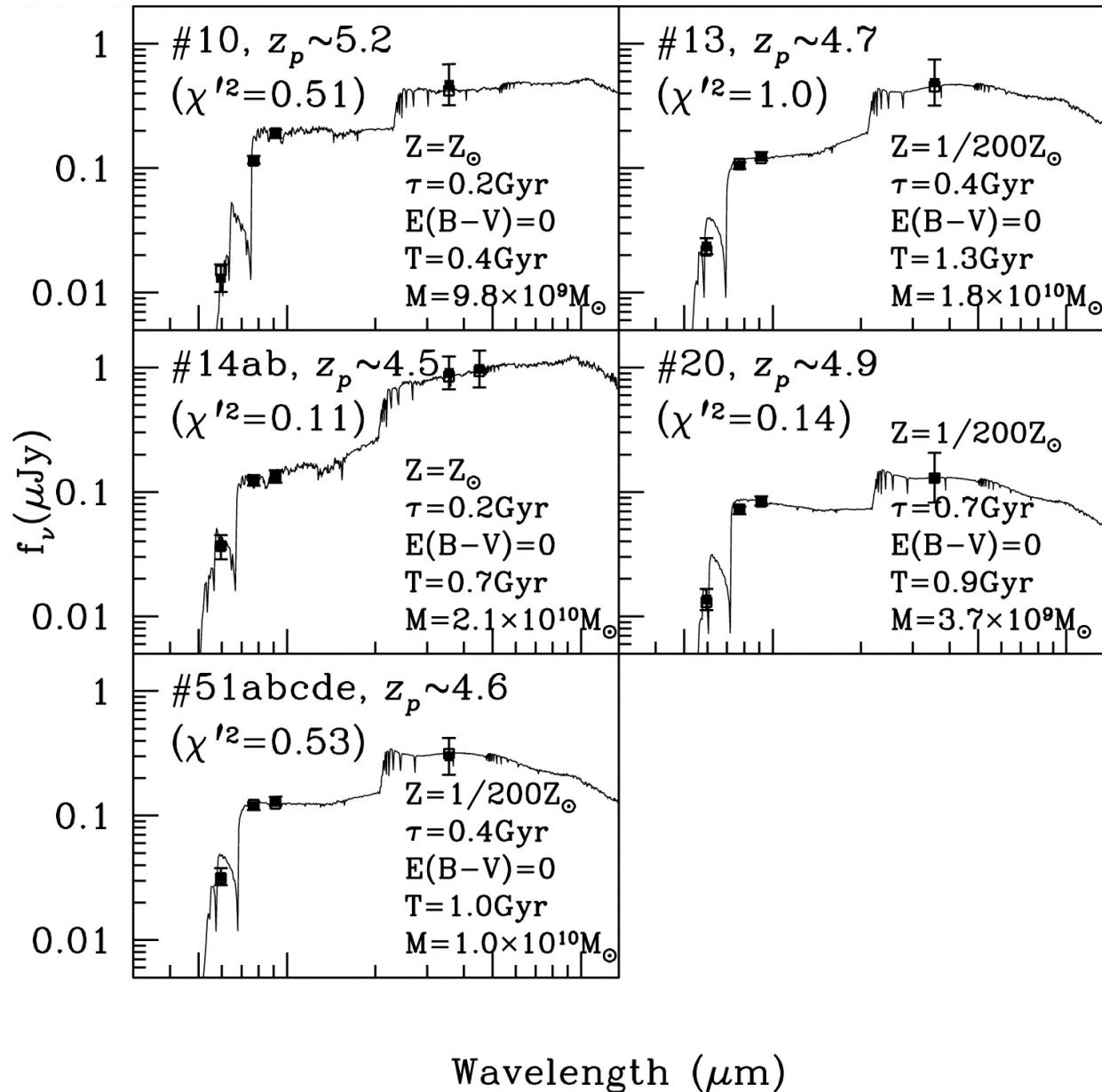
Fig. 6. from RestFrame UltraviolettoOptical Properties of Galaxies at z \sim 6 and z \sim 5 in the Hubble Ultra Deep Field: From Hubble to Spitzer Yan et al. 2005 ApJ 634 109 doi:10.1086/491695 https://dx.doi.org/10.1086/491695
