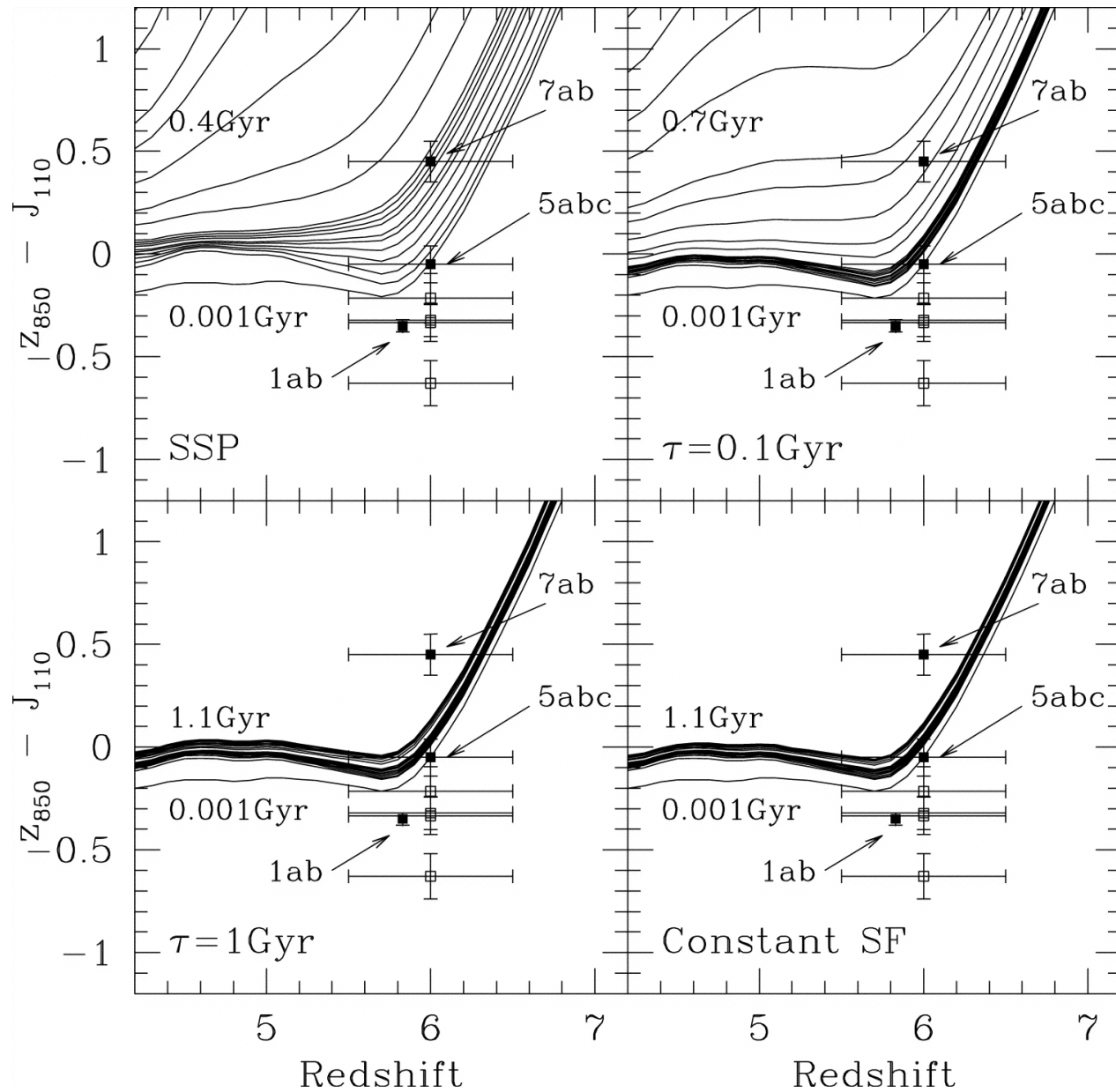
Fig. 4. from RestFrame UltraviolettoOptical Properties of Galaxies at z \sim 6 and z \sim 5 in the Hubble Ultra Deep Field: From Hubble to Spitzer Yan et al. 2005 ApJ 634 109 doi:10.1086/491695 https://dx.doi.org/10.1086/491695 © 2005. The American Astronomical Society. All rights reserved. Printed in U.S.A.
