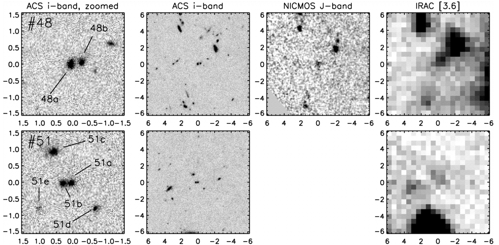
Fig. 2. from RestFrame UltraviolettoOptical Properties of Galaxies at z \sim 6 and z \sim 5 in the Hubble Ultra Deep Field: From Hubble to Spitzer Yan et al. 2005 ApJ 634 109 doi:10.1086/491695 https://dx.doi.org/10.1086/491695
