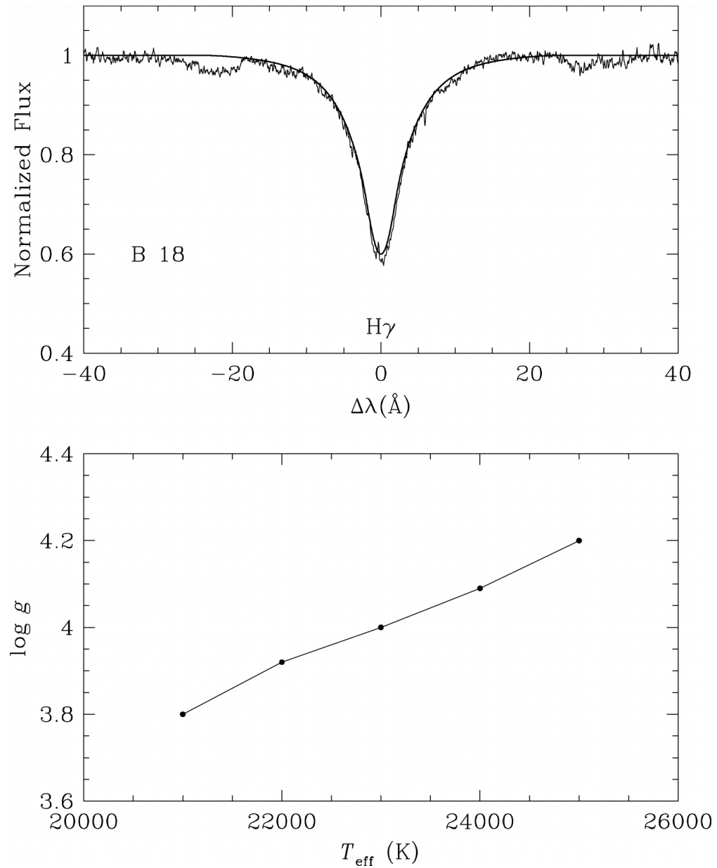
Fig. 2. from Pristine CNO Abundances from Magellanic Cloud B Stars. II. Fast Rotators in the Large Magellanic Cloud Cluster NGC 2004 Korn et al. 2005 ApJ 633 899 doi:10.1086/491619 https://dx.doi.org/10.1086/491619 © 2005. The American Astronomical Society. All rights reserved. Printed in U.S.A.
