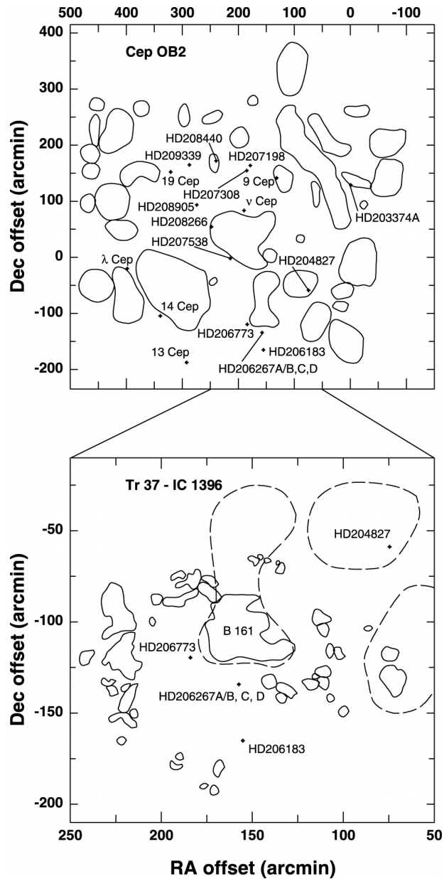
Fig. 8. from Cloud Structure and Physical Conditions in Starforming Regions from Optical Observations. II. Analysis Pan et al. 2005 ApJ 633 986 doi:10.1086/491466 https://dx.doi.org/10.1086/491466
