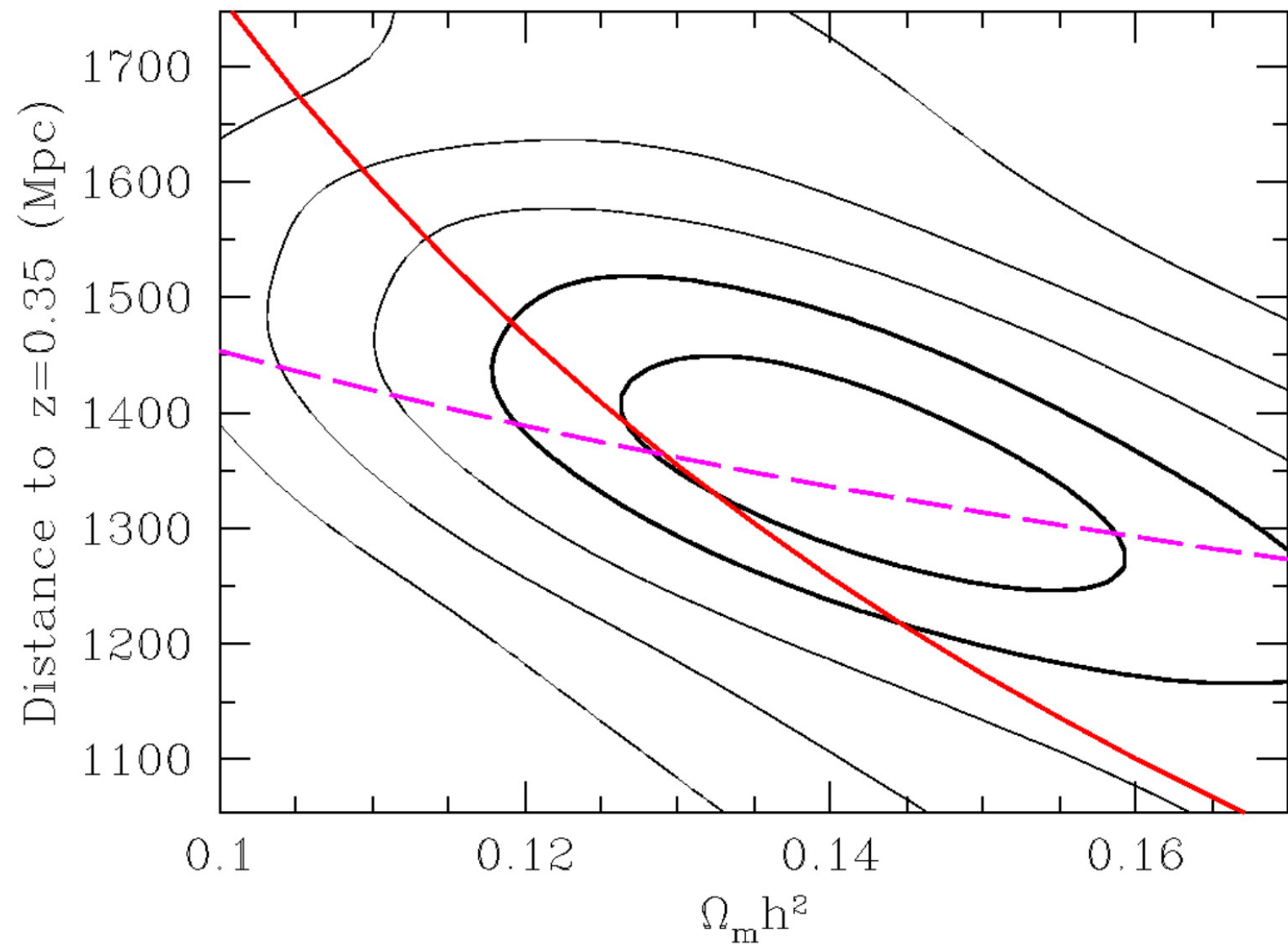
Fig. 9. from Detection of the Baryon Acoustic Peak in the LargeScale Correlation Function of SDSS Luminous Red Galaxies Eisenstein et al. 2005 ApJ 633 560 doi:10.1086/466512 https://dx.doi.org/10.1086/466512 © 2005. The American Astronomical Society. All rights reserved. Printed in U.S.A.
