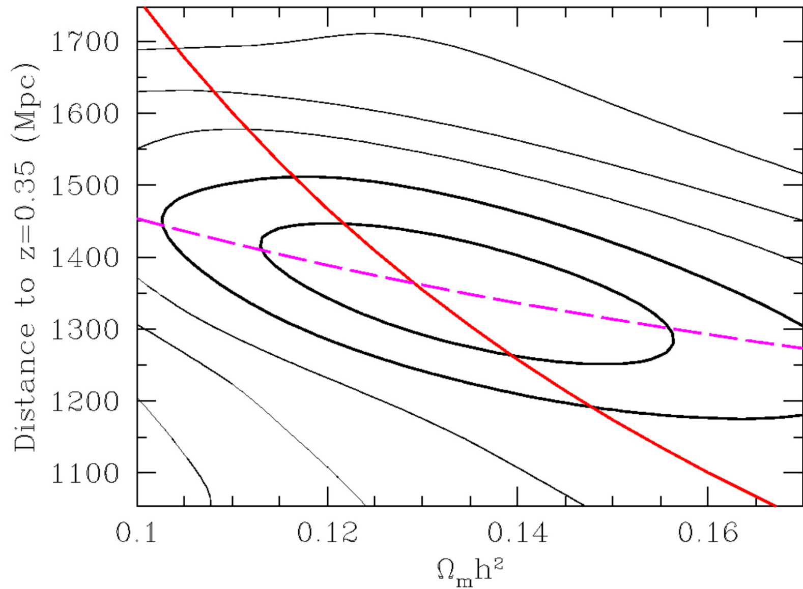
Fig. 8. from Detection of the Baryon Acoustic Peak in the LargeScale Correlation Function of SDSS Luminous Red Galaxies Eisenstein et al. 2005 ApJ 633 560 doi:10.1086/466512 https://dx.doi.org/10.1086/466512 © 2005. The American Astronomical Society. All rights reserved. Printed in U.S.A.
