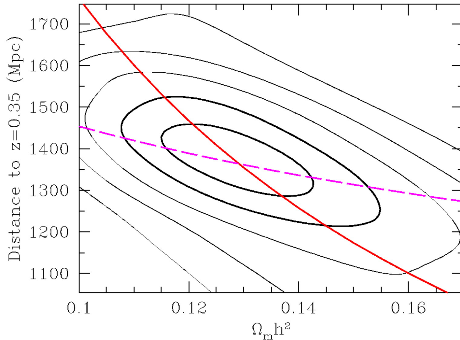
Fig. 7. from Detection of the Baryon Acoustic Peak in the LargeScale Correlation Function of SDSS Luminous Red Galaxies Eisenstein et al. 2005 ApJ 633 560 doi:10.1086/466512 https://dx.doi.org/10.1086/466512 © 2005. The American Astronomical Society. All rights reserved. Printed in U.S.A.
