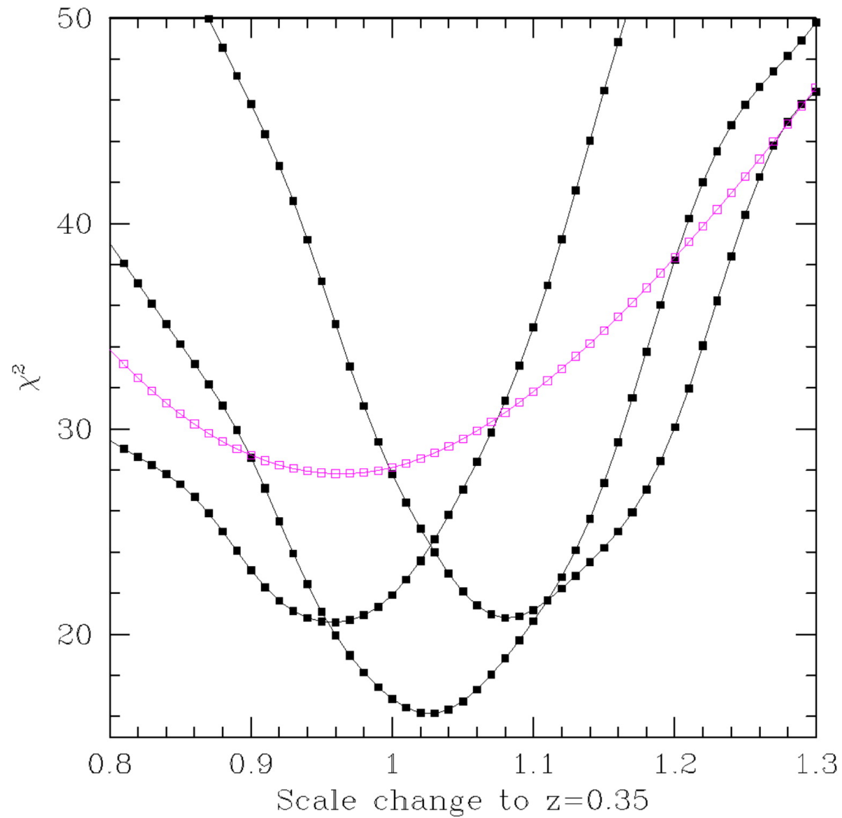
Fig. 6. from Detection of the Baryon Acoustic Peak in the LargeScale Correlation Function of SDSS Luminous Red Galaxies Eisenstein et al. 2005 ApJ 633 560 doi:10.1086/466512 https://dx.doi.org/10.1086/466512 © 2005. The American Astronomical Society. All rights reserved. Printed in U.S.A.
