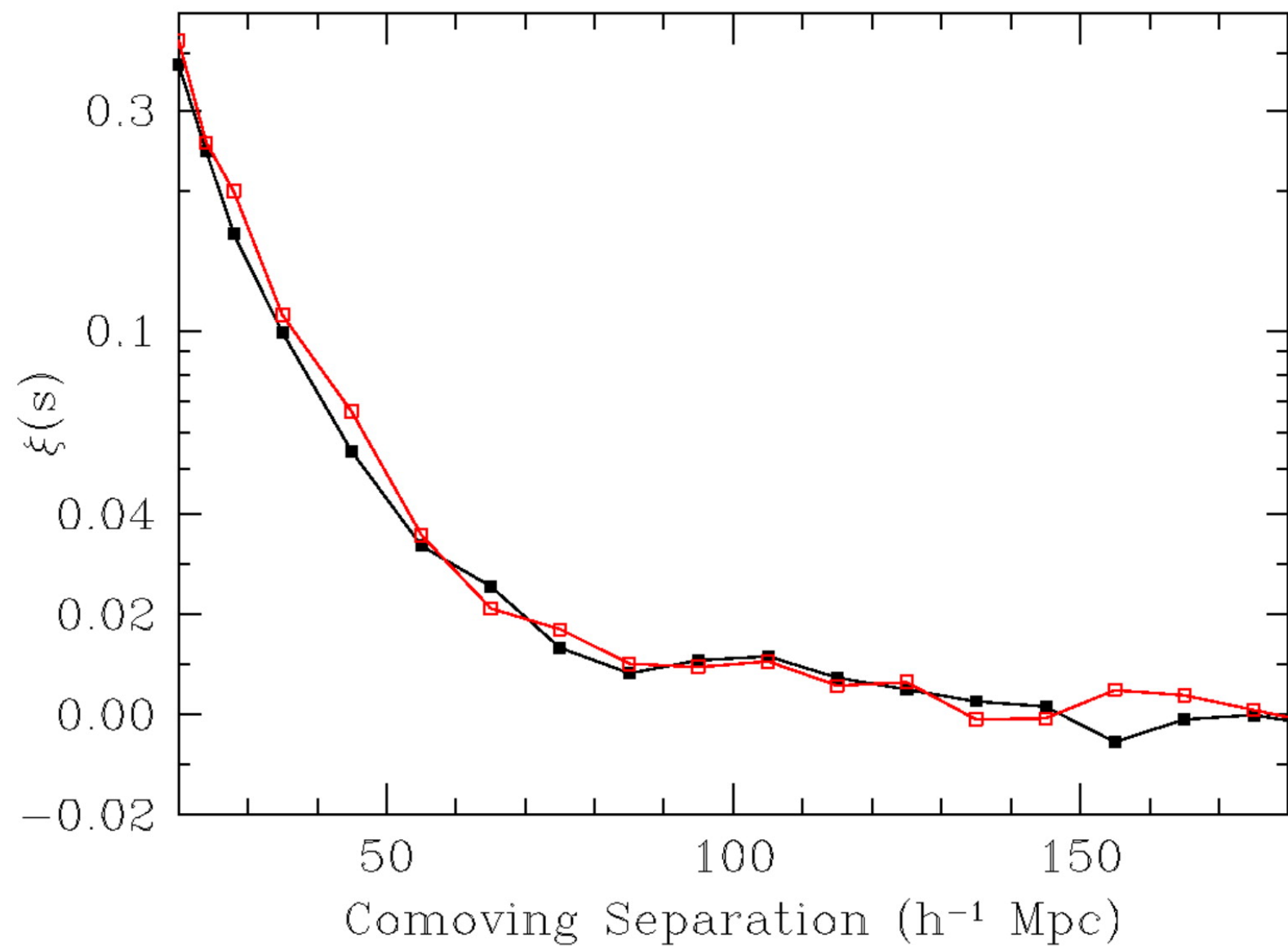
Fig. 4. from Detection of the Baryon Acoustic Peak in the LargeScale Correlation Function of SDSS Luminous Red Galaxies Eisenstein et al. 2005 ApJ 633 560 doi:10.1086/466512 https://dx.doi.org/10.1086/466512 © 2005. The American Astronomical Society. All rights reserved. Printed in U.S.A.
