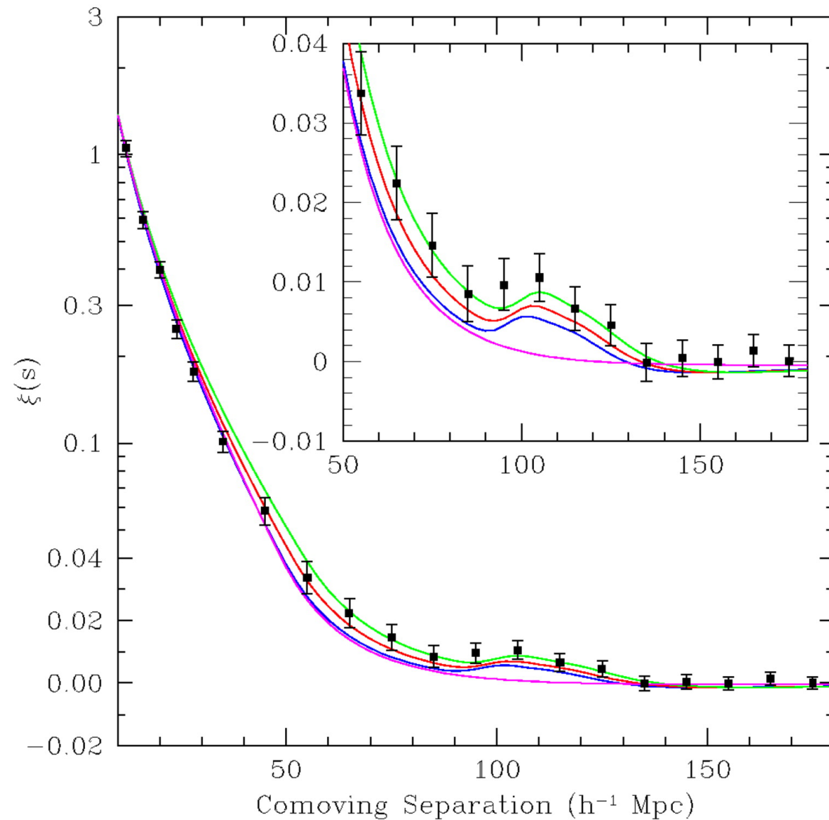
Fig. 2. from Detection of the Baryon Acoustic Peak in the LargeScale Correlation Function of SDSS Luminous Red Galaxies Eisenstein et al. 2005 ApJ 633 560 doi:10.1086/466512 https://dx.doi.org/10.1086/466512 © 2005. The American Astronomical Society. All rights reserved. Printed in U.S.A.
