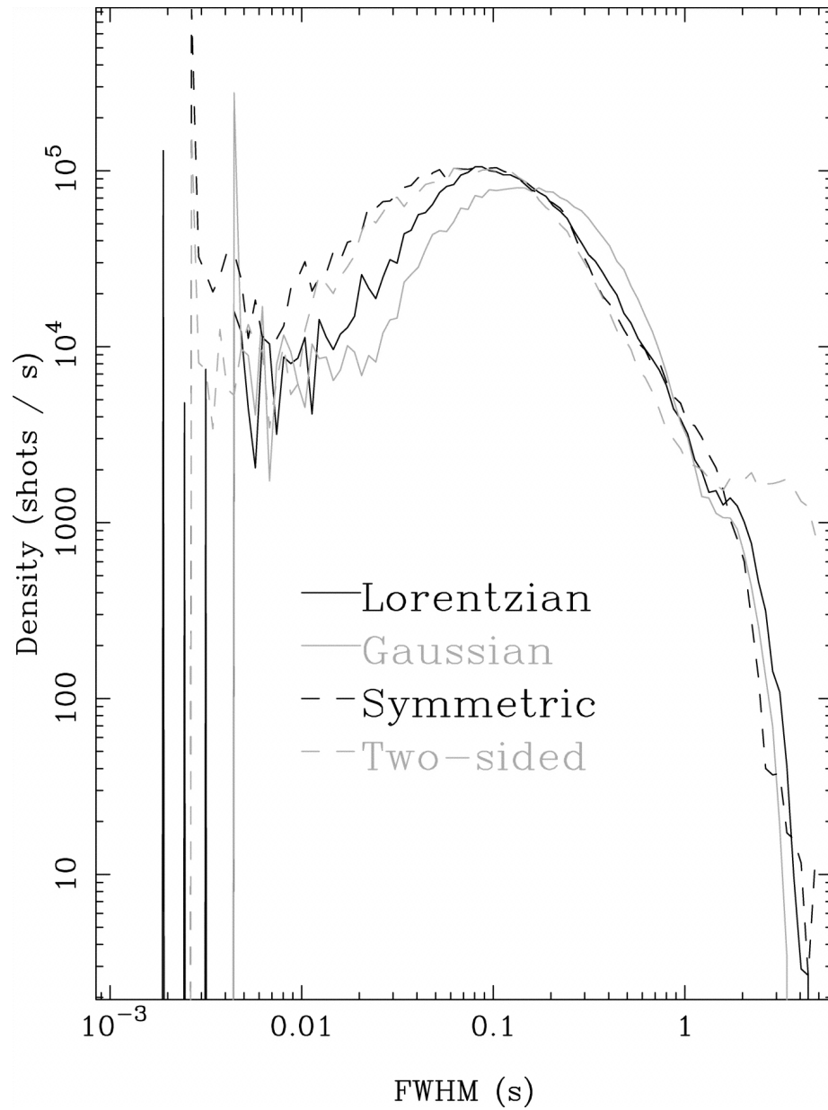
Fig. 9. from Time Domain Studies of XRay Shot Noise in Cygnus X1 Focke, Wai, & Swank 2005 ApJ 633 1085 doi:10.1086/462407 https://dx.doi.org/10.1086/462407 Copyright is not claimed for this article. Printed in U.S.A.
