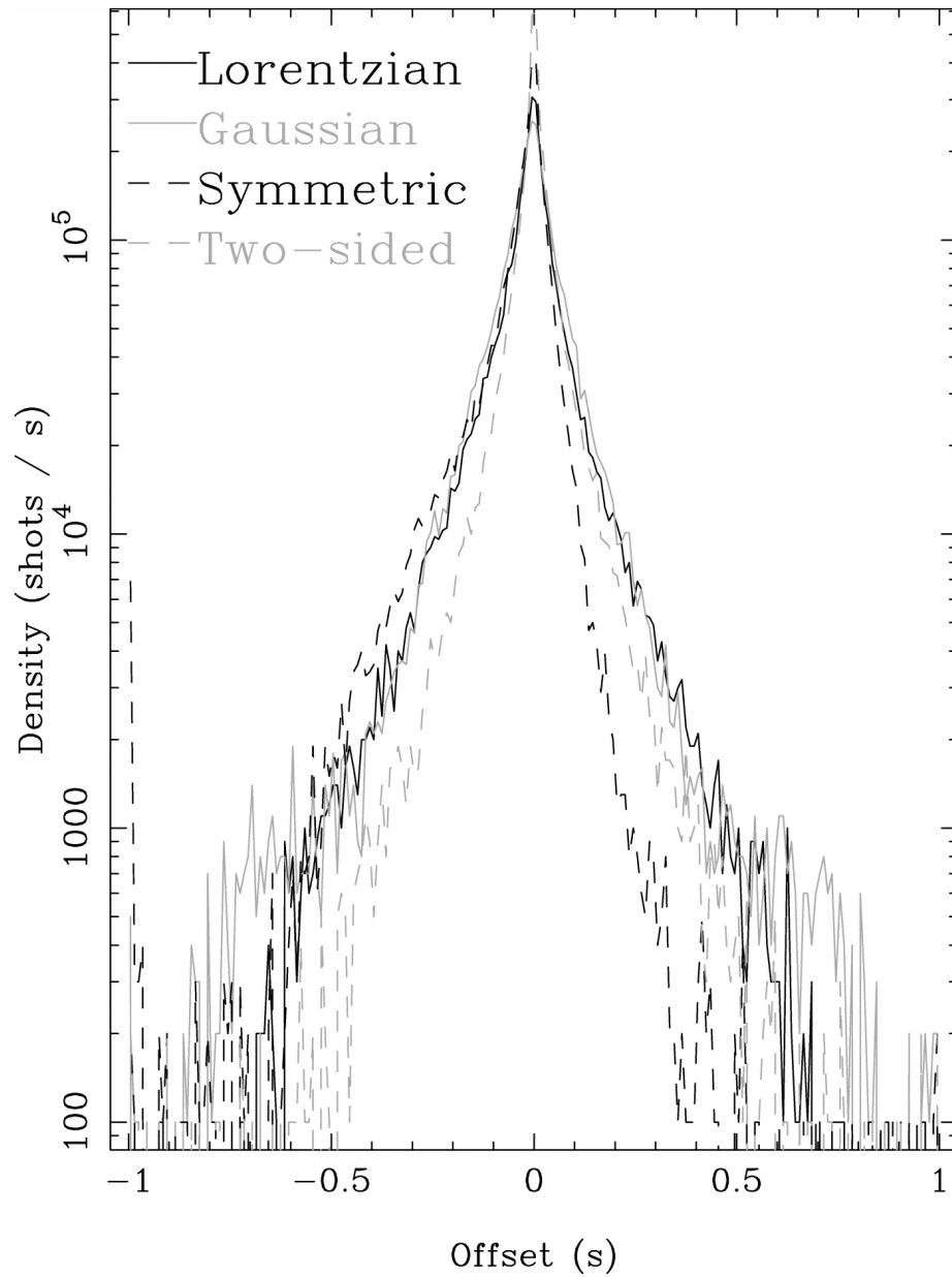
Fig. 8. from Time Domain Studies of XRay Shot Noise in Cygnus X1 Focke, Wai, & Swank 2005 ApJ 633 1085 doi:10.1086/462407 https://dx.doi.org/10.1086/462407 Copyright is not claimed for this article. Printed in U.S.A.
