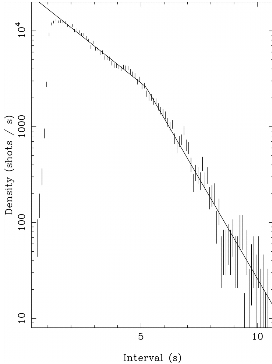
Fig. 2. from Time Domain Studies of XRay Shot Noise in Cygnus X1 Focke, Wai, & Swank 2005 ApJ 633 1085 doi:10.1086/462407 https://dx.doi.org/10.1086/462407 Copyright is not claimed for this article. Printed in U.S.A.
