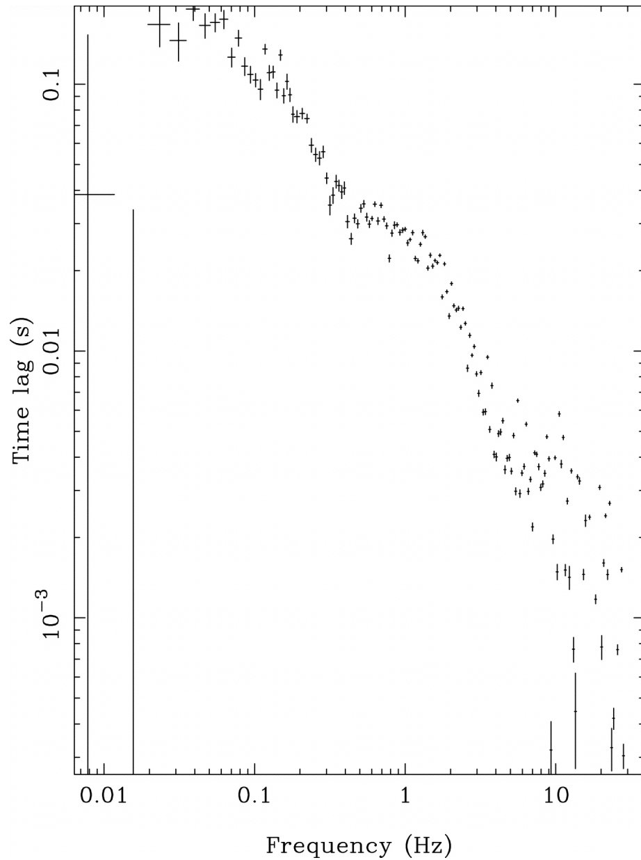
Fig. 14. from Time Domain Studies of XRay Shot Noise in Cygnus X1 Focke, Wai, & Swank 2005 ApJ 633 1085 doi:10.1086/462407 https://dx.doi.org/10.1086/462407 Copyright is not claimed for this article. Printed in U.S.A.
