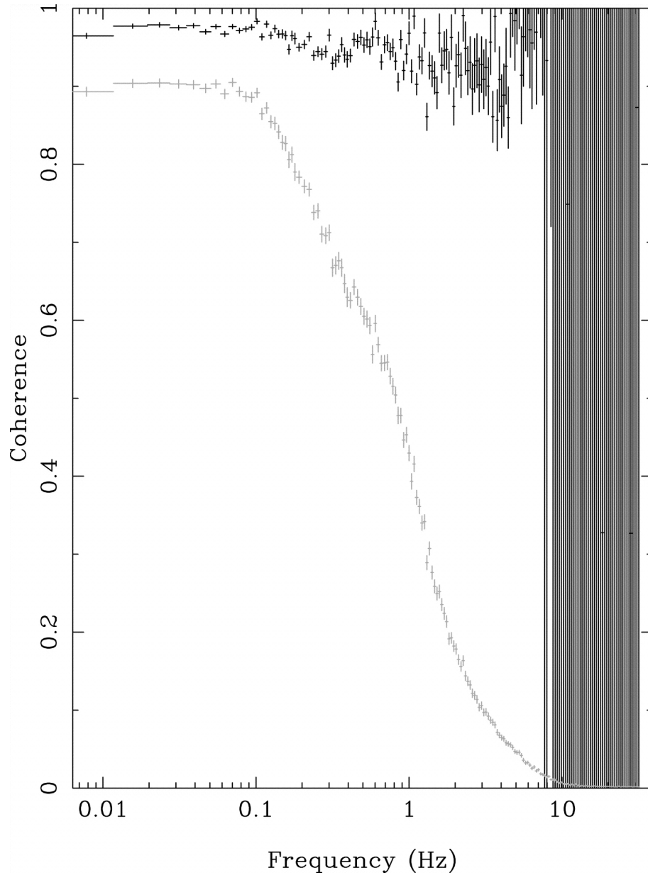
Fig. 13. from Time Domain Studies of XRay Shot Noise in Cygnus X1 Focke, Wai, & Swank 2005 ApJ 633 1085 doi:10.1086/462407 https://dx.doi.org/10.1086/462407 Copyright is not claimed for this article. Printed in U.S.A.
