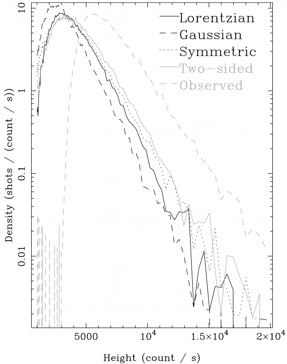
Fig. 11. from Time Domain Studies of XRay Shot Noise in Cygnus X1 Focke, Wai, & Swank 2005 ApJ 633 1085 doi:10.1086/462407 https://dx.doi.org/10.1086/462407 Copyright is not claimed for this article. Printed in U.S.A.
