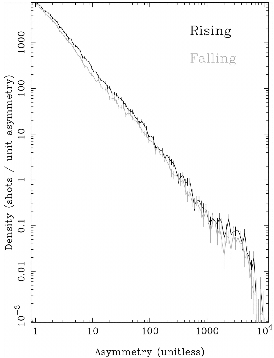
Fig. 10. from Time Domain Studies of XRay Shot Noise in Cygnus X1 Focke, Wai, & Swank 2005 ApJ 633 1085 doi:10.1086/462407 https://dx.doi.org/10.1086/462407 Copyright is not claimed for this article. Printed in U.S.A.
