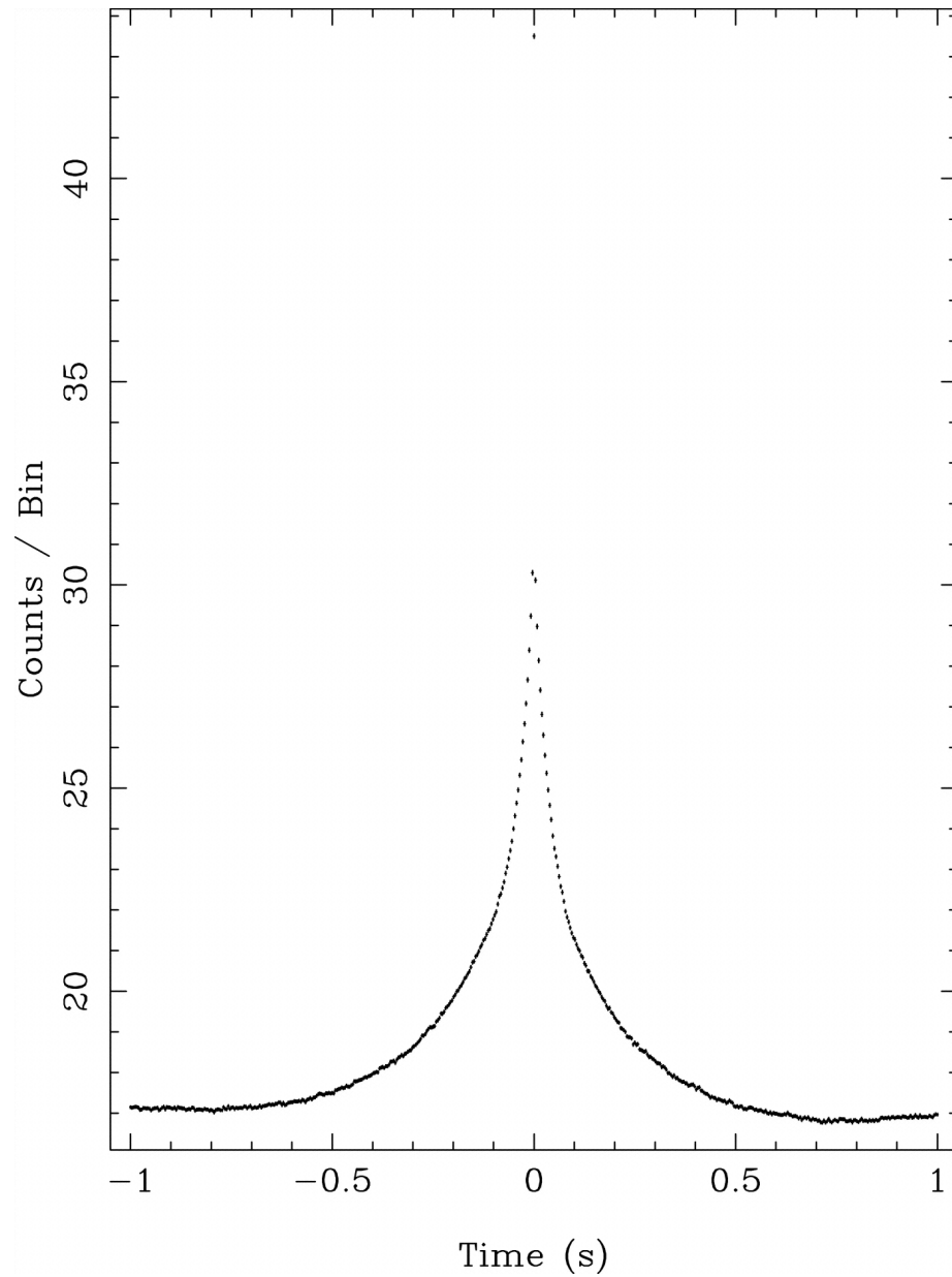
Fig. 1. from Time Domain Studies of XRay Shot Noise in Cygnus X1 Focke, Wai, & Swank 2005 ApJ 633 1085 doi:10.1086/462407 https://dx.doi.org/10.1086/462407 Copyright is not claimed for this article. Printed in U.S.A.
