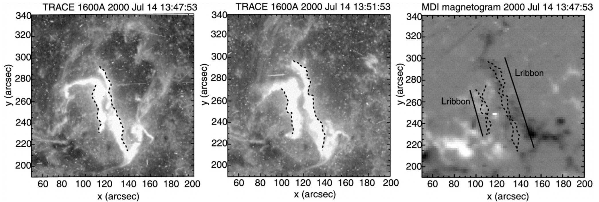
Fig. 9. from Measurement of the Energy Release Rate and the Reconnection Rate in Solar Flares Isobe, Takasaki, & Shibata 2005 ApJ 632 1184 doi:10.1086/444490 https://dx.doi.org/10.1086/444490
