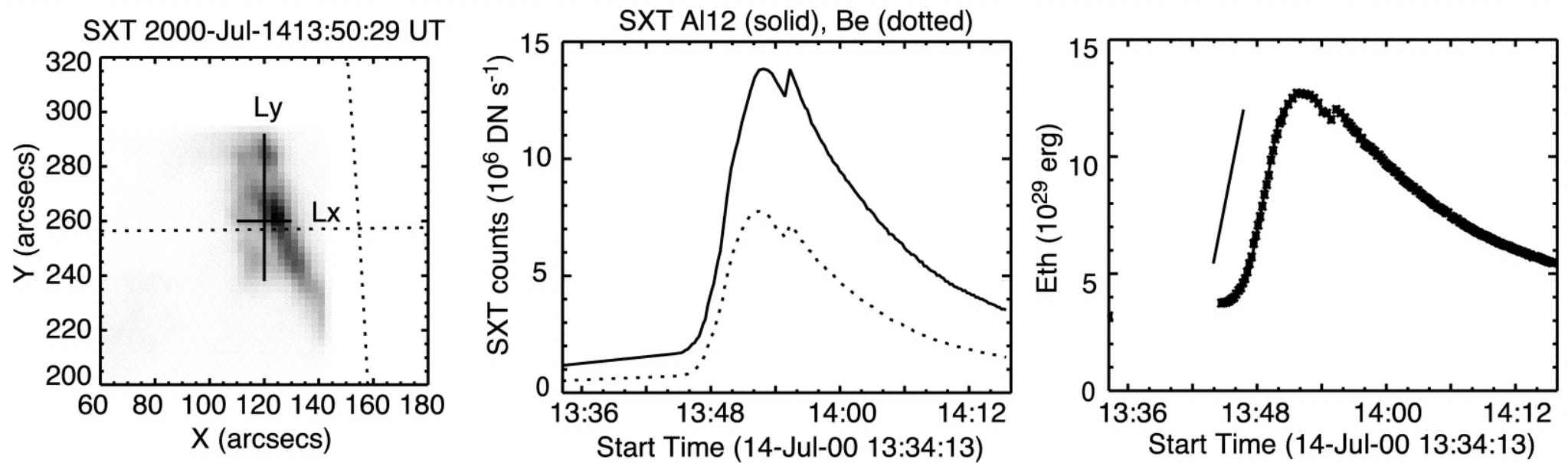
Fig. 8. from Measurement of the Energy Release Rate and the Reconnection Rate in Solar Flares Isobe, Takasaki, & Shibata 2005 ApJ 632 1184 doi:10.1086/444490 https://dx.doi.org/10.1086/444490 © 2005. The American Astronomical Society. All rights reserved. Printed in U.S.A.
