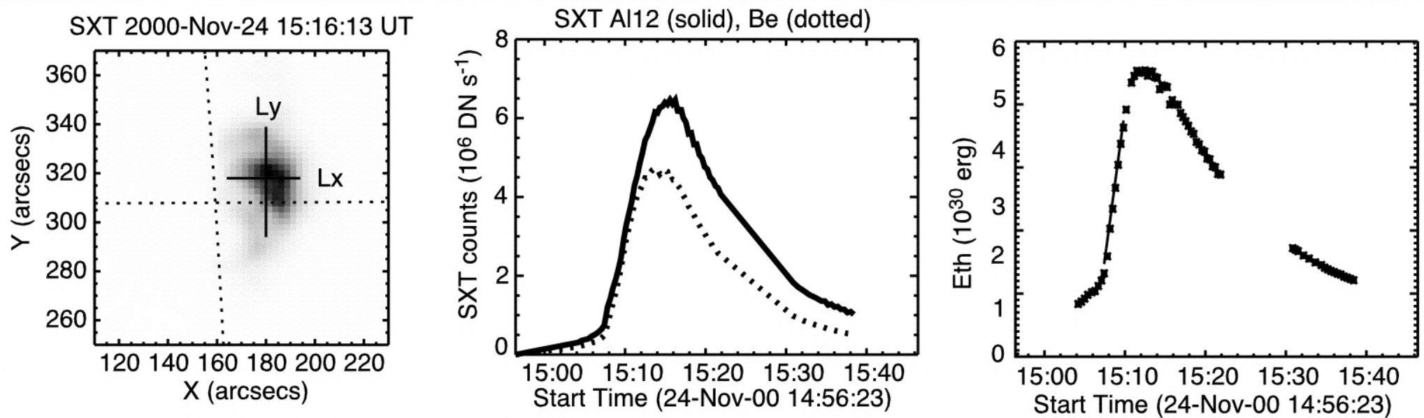
Fig. 6. from Measurement of the Energy Release Rate and the Reconnection Rate in Solar Flares Isobe, Takasaki, & Shibata 2005 ApJ 632 1184 doi:10.1086/444490 https://dx.doi.org/10.1086/444490 © 2005. The American Astronomical Society. All rights reserved. Printed in U.S.A.
