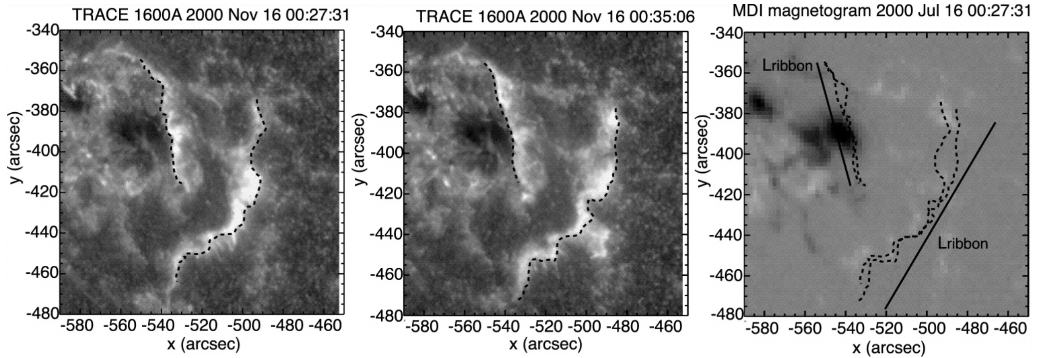
Fig. 11. from Measurement of the Energy Release Rate and the Reconnection Rate in Solar Flares Isobe, Takasaki, & Shibata 2005 ApJ 632 1184 doi:10.1086/444490 https://dx.doi.org/10.1086/444490
