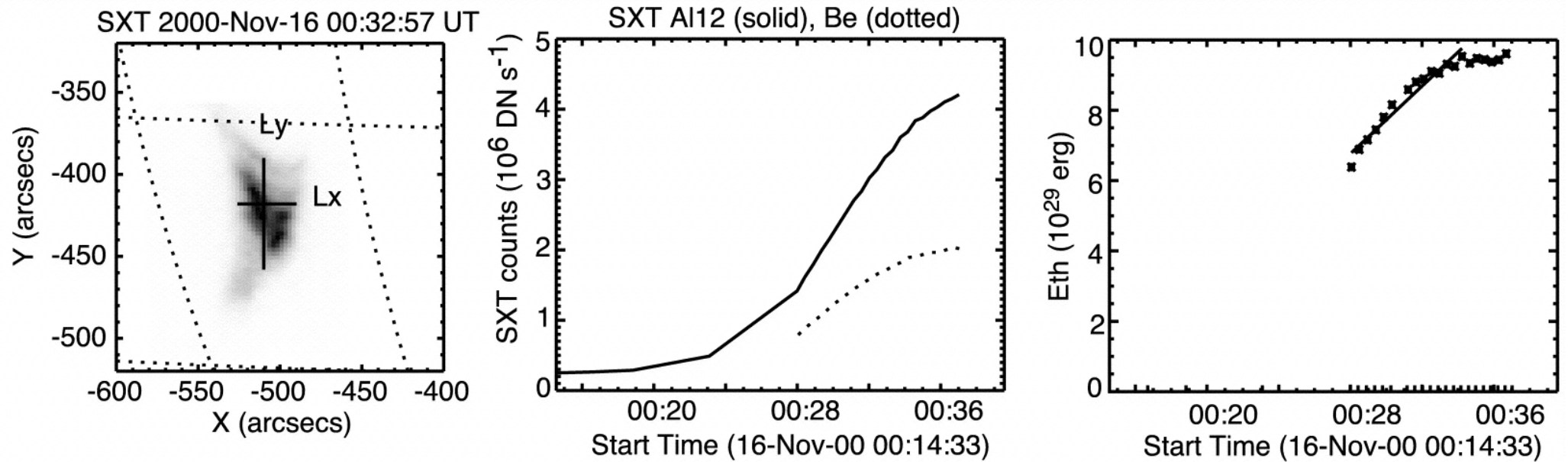
Fig. 10. from Measurement of the Energy Release Rate and the Reconnection Rate in Solar Flares Isobe, Takasaki, & Shibata 2005 ApJ 632 1184 doi:10.1086/444490 https://dx.doi.org/10.1086/444490 © 2005. The American Astronomical Society. All rights reserved. Printed in U.S.A.
