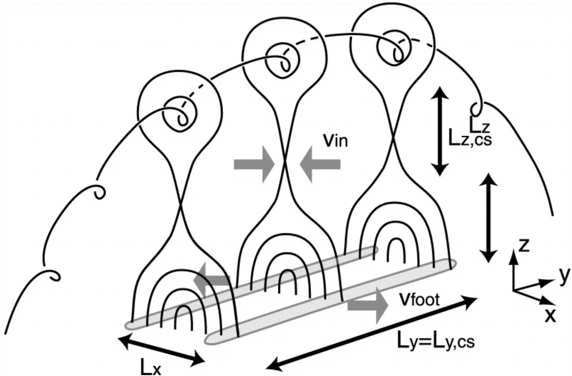
Fig. 1. from Measurement of the Energy Release Rate and the Reconnection Rate in Solar Flares Isobe, Takasaki, & Shibata 2005 ApJ 632 1184 doi:10.1086/444490 https://dx.doi.org/10.1086/444490 © 2005. The American Astronomical Society. All rights reserved. Printed in U.S.A.
