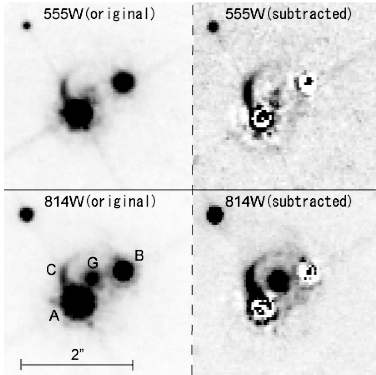
Fig. 8. from SDSS J024634.11082536.2: A New Gravitationally Lensed Quasar from the Sloan Digital Sky Survey Inada et al. 2005 AJ 130 1967 doi:10.1086/432930 https://dx.doi.org/10.1086/432930 © 2005. The American Astronomical Society. All rights reserved. Printed in U.S.A.
