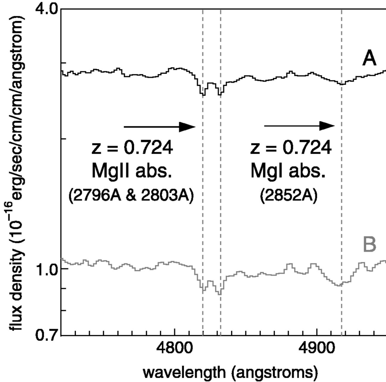
Fig. 7. from SDSS J024634.11082536.2: A New Gravitationally Lensed Quasar from the Sloan Digital Sky Survey Inada et al. 2005 AJ 130 1967 doi:10.1086/432930 https://dx.doi.org/10.1086/432930 © 2005. The American Astronomical Society. All rights reserved. Printed in U.S.A.
