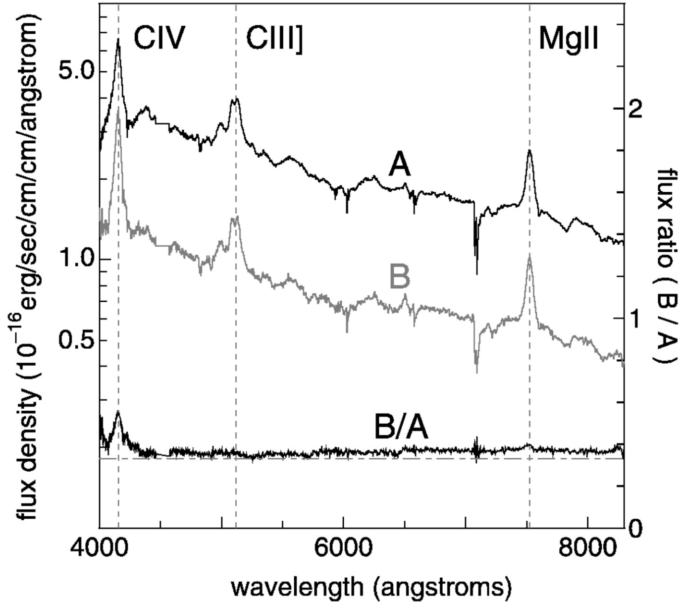
Fig. 6. from SDSS J024634.11082536.2: A New Gravitationally Lensed Quasar from the Sloan Digital Sky Survey Inada et al. 2005 AJ 130 1967 doi:10.1086/432930 https://dx.doi.org/10.1086/432930 © 2005. The American Astronomical Society. All rights reserved. Printed in U.S.A.
