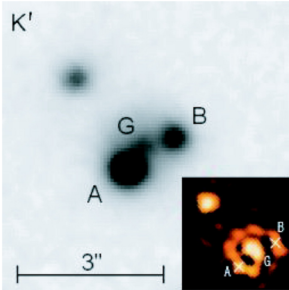
Fig. 5. from SDSS J024634.11082536.2: A New Gravitationally Lensed Quasar from the Sloan Digital Sky Survey Inada et al. 2005 AJ 130 1967 doi:10.1086/432930 https://dx.doi.org/10.1086/432930 © 2005. The American Astronomical Society. All rights reserved. Printed in U.S.A.
