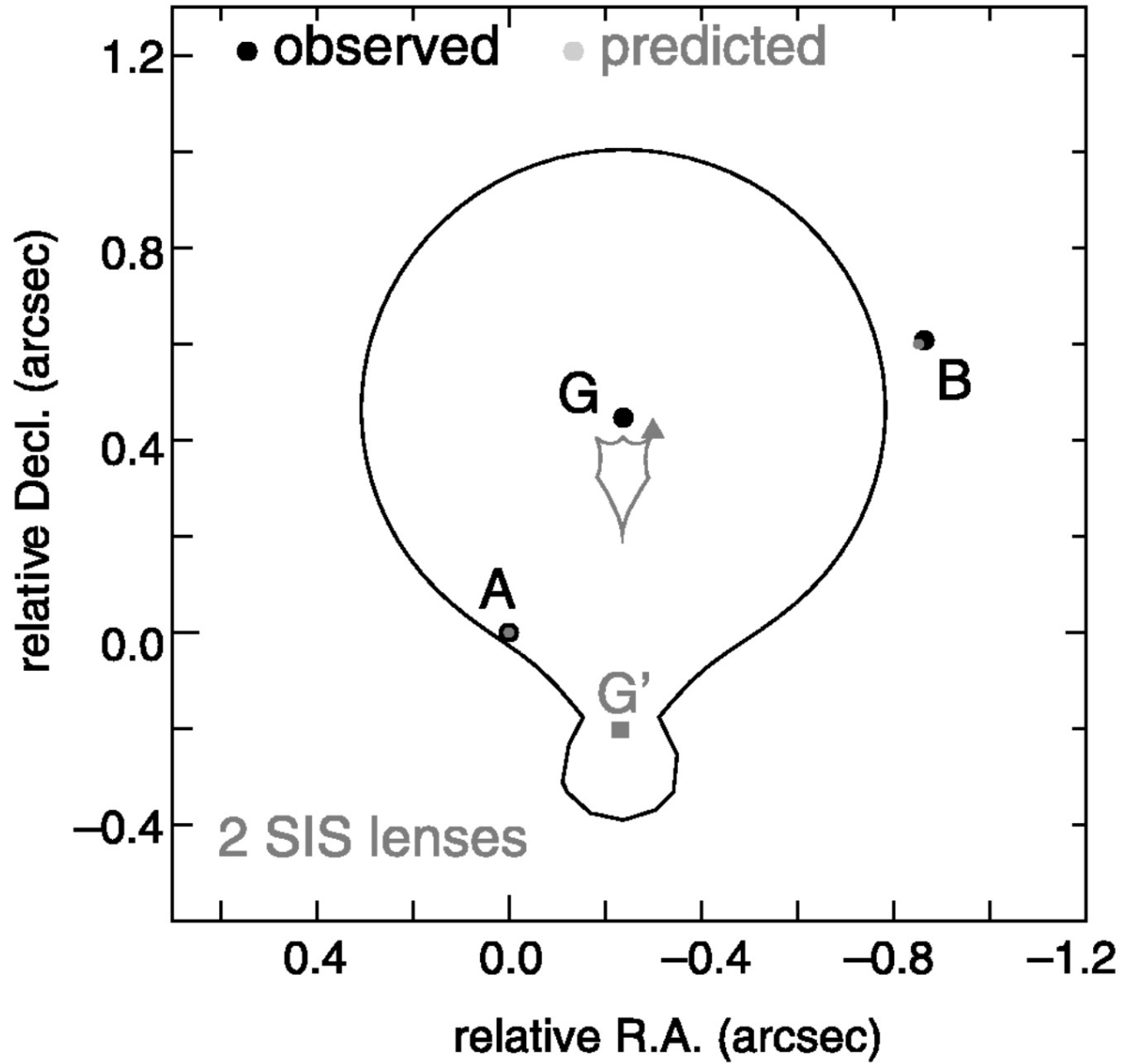
Fig. 11. from SDSS J024634.11082536.2: A New Gravitationally Lensed Quasar from the Sloan Digital Sky Survey Inada et al. 2005 AJ 130 1967 doi:10.1086/432930 https://dx.doi.org/10.1086/432930 © 2005. The American Astronomical Society. All rights reserved. Printed in U.S.A.
