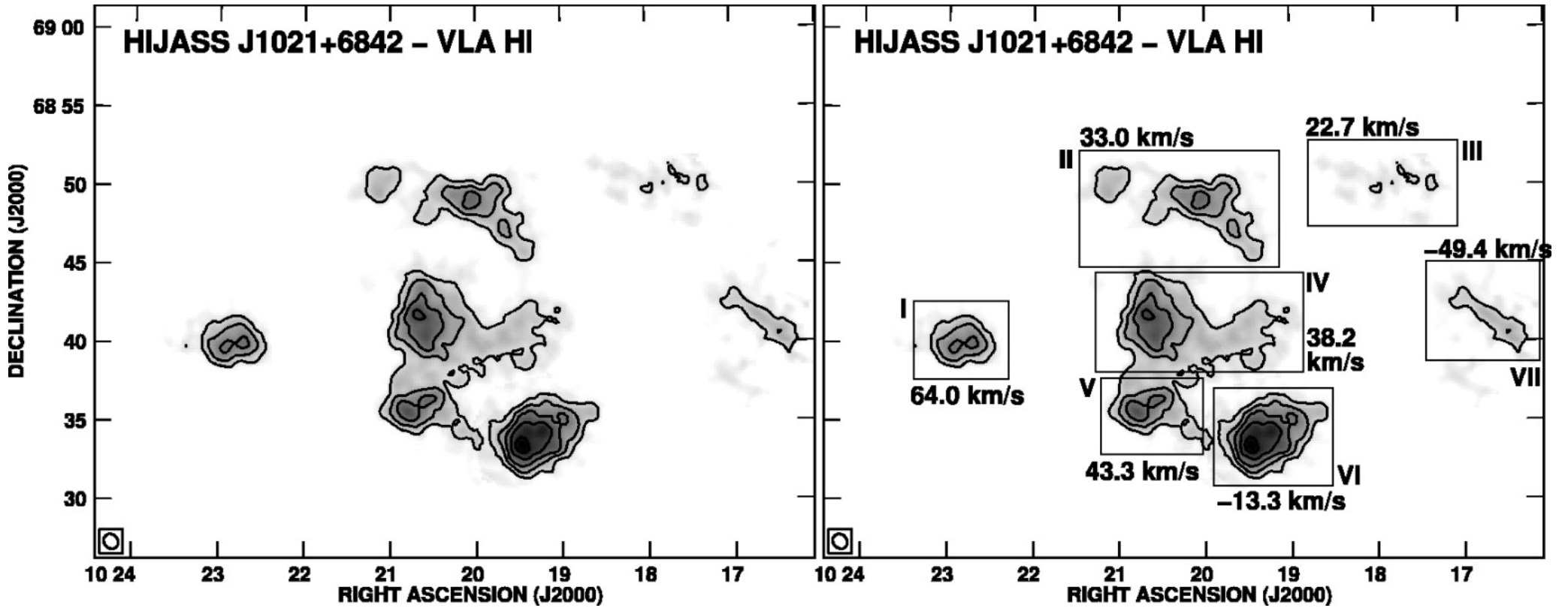
Fig. 2. from VLA Imaging of the Intriguing H I Cloud HIJASS J1021+6842 in the M81 Group Walter, Skillman, & Brinks 2005 ApJL 627 L105 doi:10.1086/432417 https://dx.doi.org/10.1086/432417
