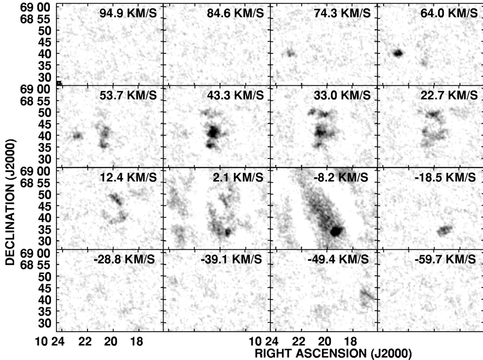
Fig. 1. from VLA Imaging of the Intriguing H I Cloud HIJASS J1021+6842 in the M81 Group Walter, Skillman, & Brinks 2005 ApJL 627 L105 doi:10.1086/432417 https://dx.doi.org/10.1086/432417
