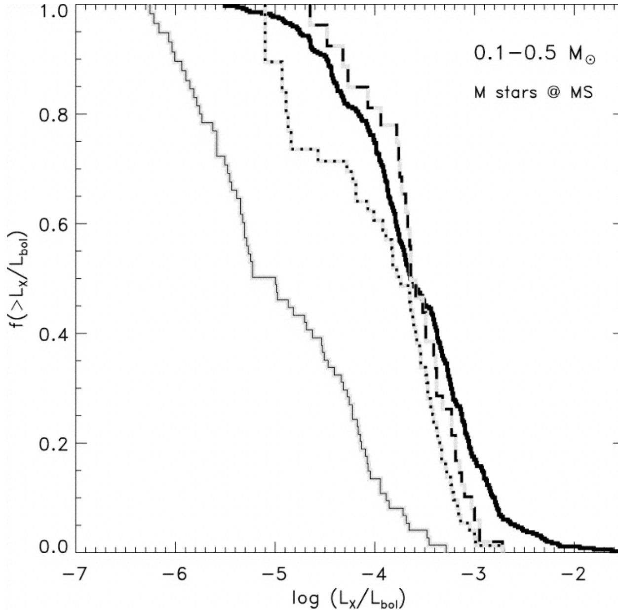
Fig. 5. from The Evolution of XRay Emission in Young Stars Preibisch & Feigelson 2005 ApJS 160 390 doi:10.1086/432094 https://dx.doi.org/10.1086/432094
