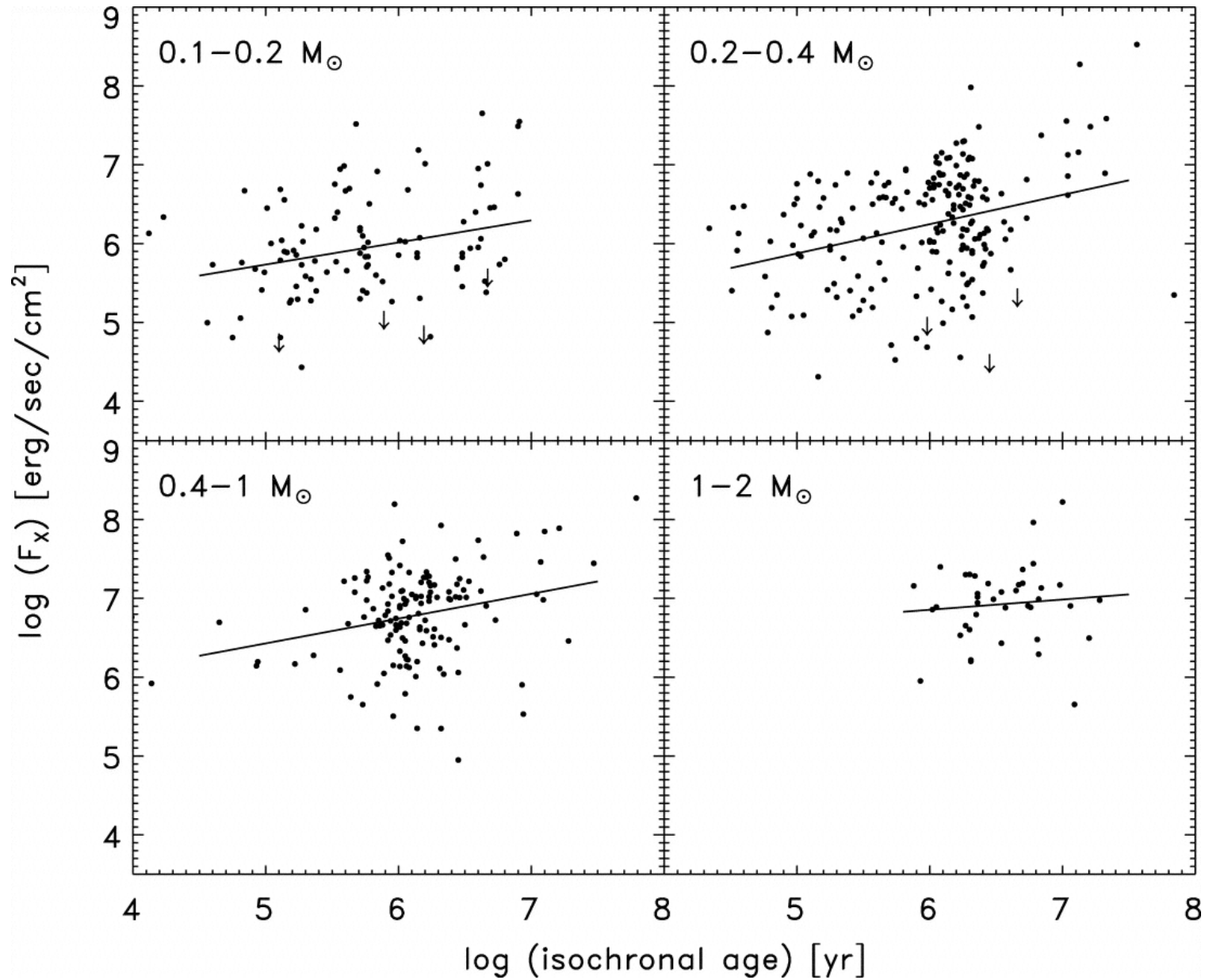
Fig. 3. from The Evolution of XRay Emission in Young Stars Preibisch & Feigelson 2005 ApJS 160 390 doi:10.1086/432094 https://dx.doi.org/10.1086/432094
