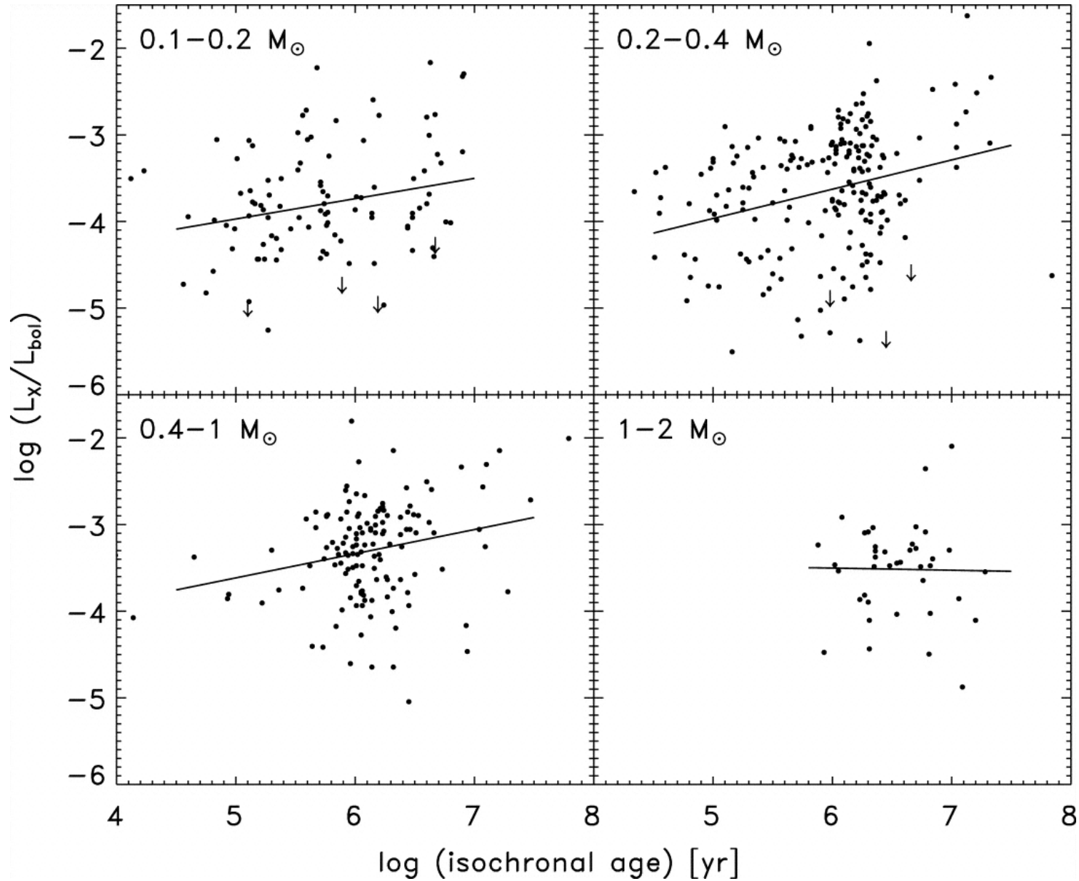
Fig. 2. from The Evolution of XRay Emission in Young Stars Preibisch & Feigelson 2005 ApJS 160 390 doi:10.1086/432094 https://dx.doi.org/10.1086/432094
