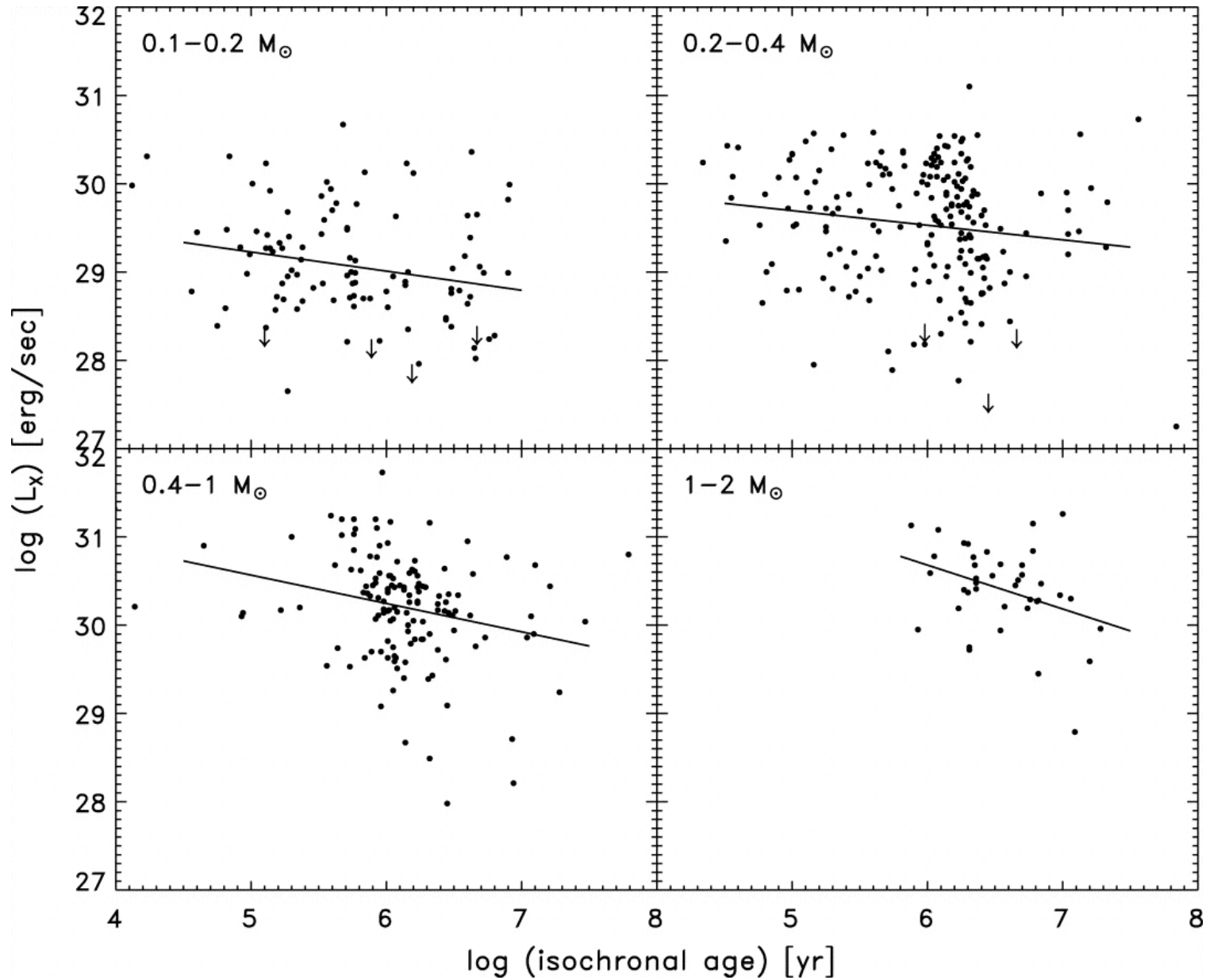
Fig. 1. from The Evolution of XRay Emission in Young Stars Preibisch & Feigelson 2005 ApJS 160 390 doi:10.1086/432094 https://dx.doi.org/10.1086/432094
