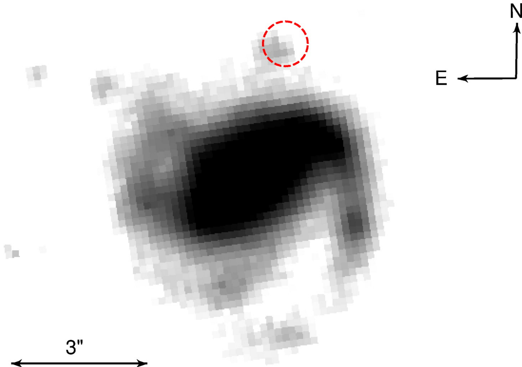
Fig. 1. from The Radio Afterglow and Host Galaxy of the Dark GRB 020819 Jakobsson et al. 2005 ApJ 629 45 doi:10.1086/431359 https://dx.doi.org/10.1086/431359 © 2005. The American Astronomical Society. All rights reserved. Printed in U.S.A.
