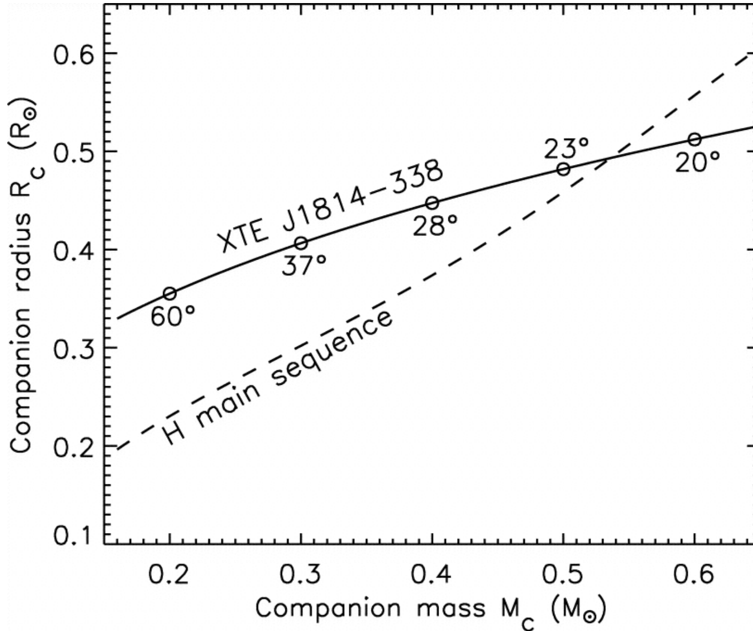
Fig. 3. from The XRay Position and Optical Counterpart of the Accretionpowered Millisecond Pulsar XTE J1814338 Krauss et al. 2005 ApJ 627 910 doi:10.1086/430595 https://dx.doi.org/10.1086/430595 © 2005. The American Astronomical Society. All rights reserved. Printed in U.S.A.
